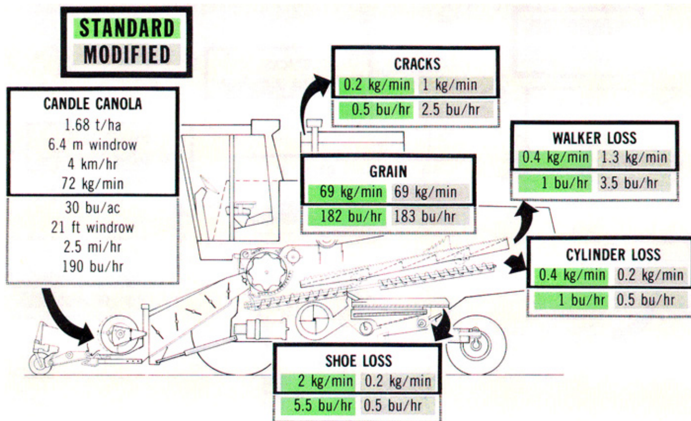
FIGURE 26. Combine Lossrates in Candle Canola.
