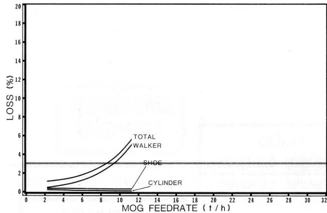
FIGURE 18. Grain Loss for the Modified Combine in Candle Canola.
