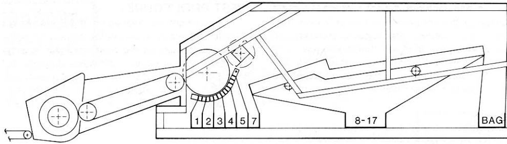
FIGURE 30. Sampling Locations.
