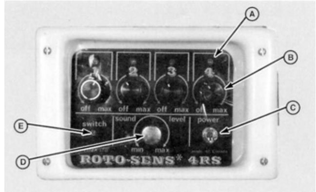
FIGURE 2. Control Box: (A) channel warning lights, (B) speed adjustment dials, (C) power switch, (D) buzzer sound level adjustment, (E) alarm switch light.
