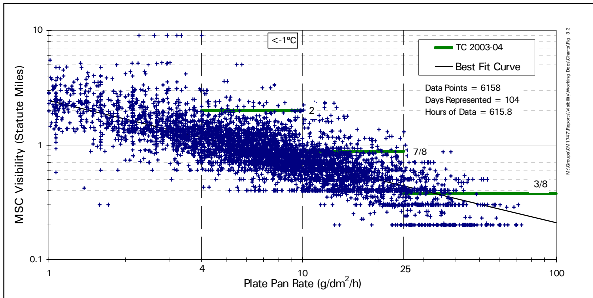
Figure 3.3: 2003-04 TC Visibility Boundaries – Below -1°C
