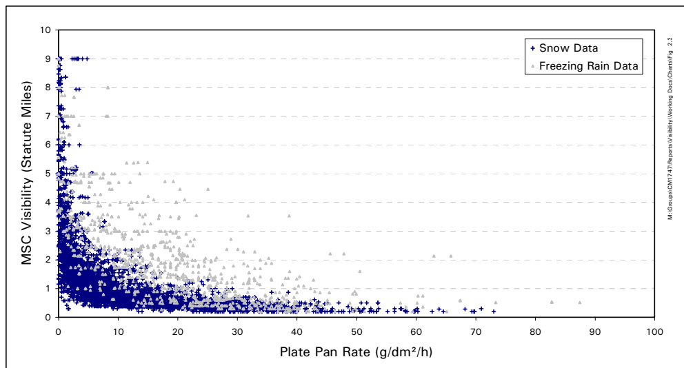
Figure 2.5: Removed Freezing Rain Data Points
