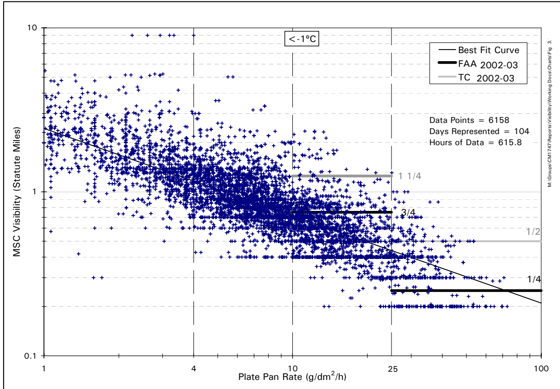
Figure 3.1: 2002-03 TC and FAA Visibility Boundaries – Below -1^\circ\text{C}
