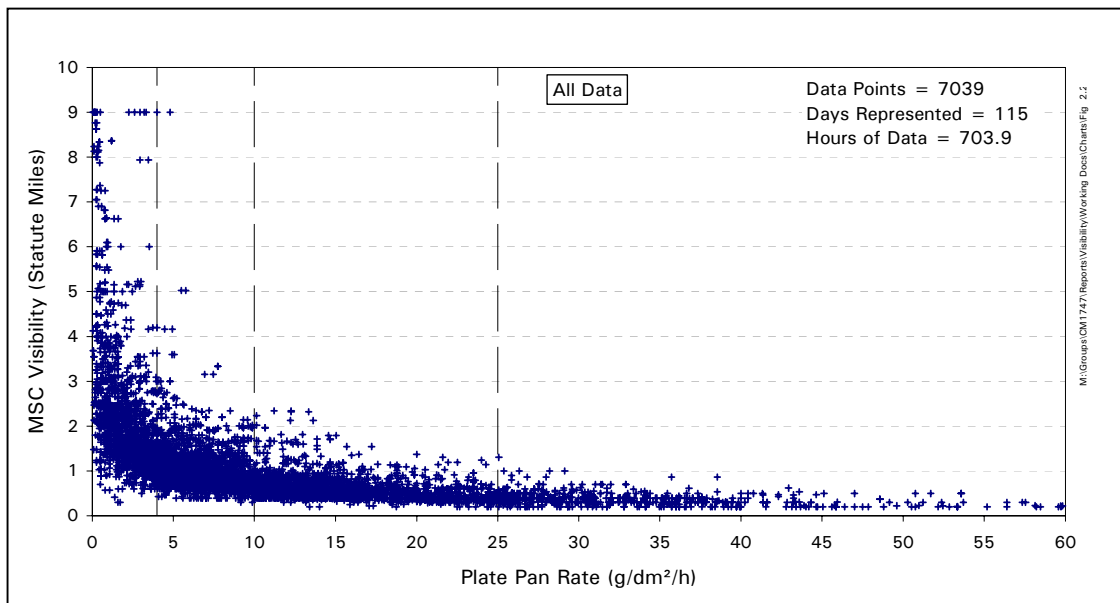
Figure 2.2: Visibility vs. Rate (1995-96 to 2001-02)
