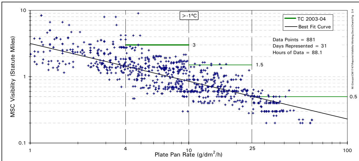
Figure 3.4: 2003-04 TC Visibility Boundaries – Above -1°C
