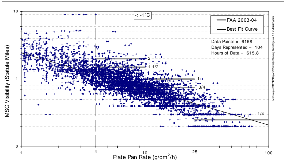
Figure 3.5: 2003-04 FAA Visibility Boundaries – Below -1°C
