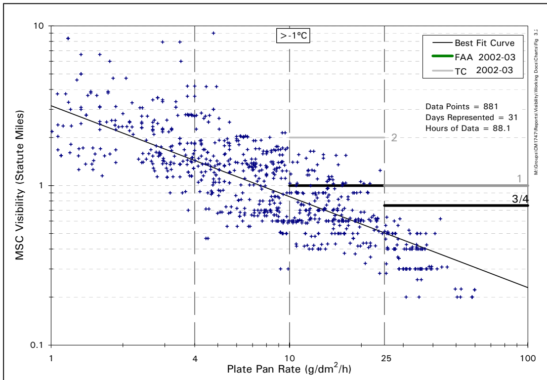
Figure 3.2: 2002-03 TC and FAA Visibility Boundaries – Above -1^\circ\text{C}
