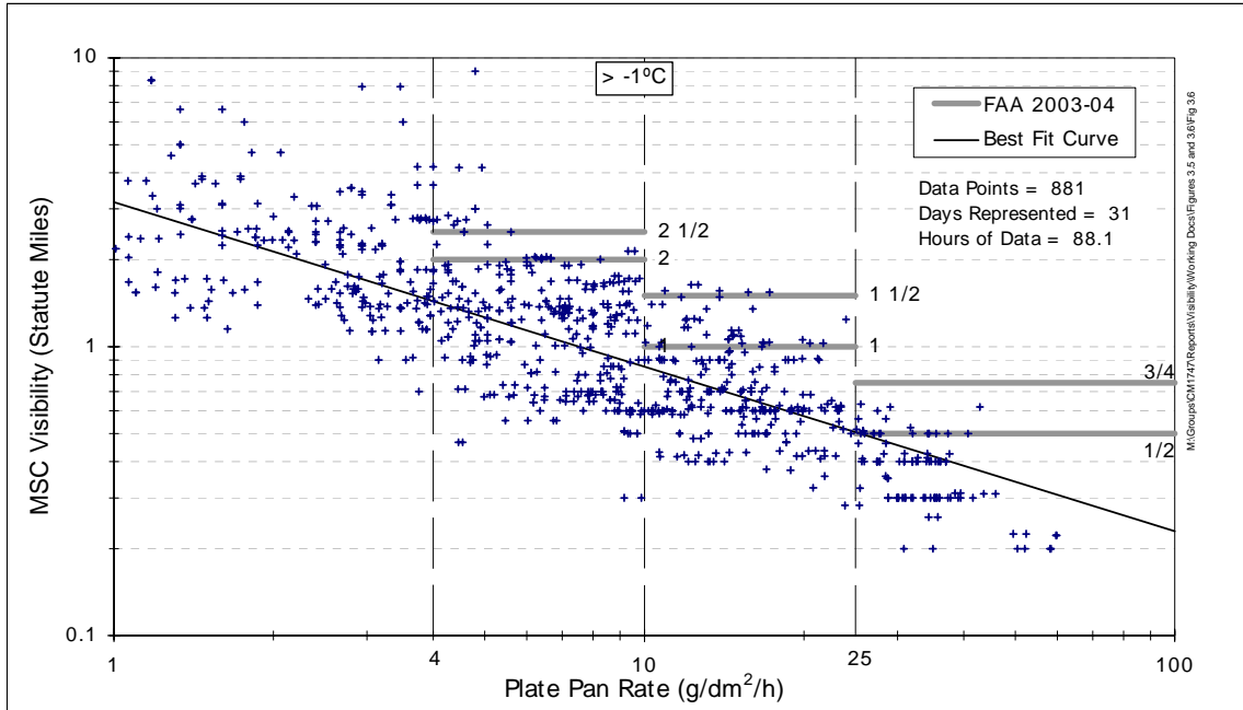
Figure 3.6: 2003-04 FAA Visibility Boundaries – Above -1°C
