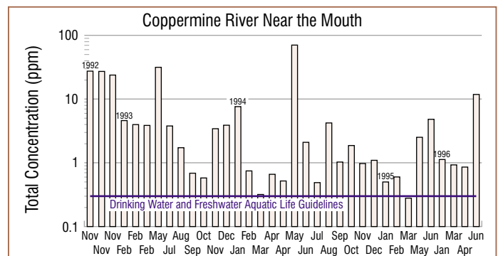
Figure 27. Total Iron Concentration.
