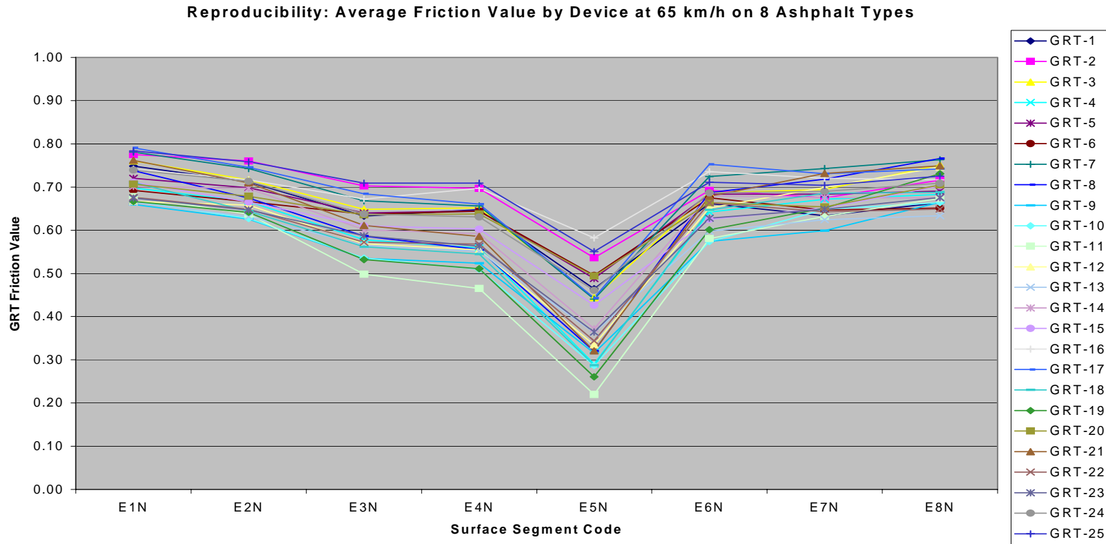
Figure 3. A sample extract of the NATAM database [7] for GripTester devices. Each friction value shown by marker is the average of three runs.
