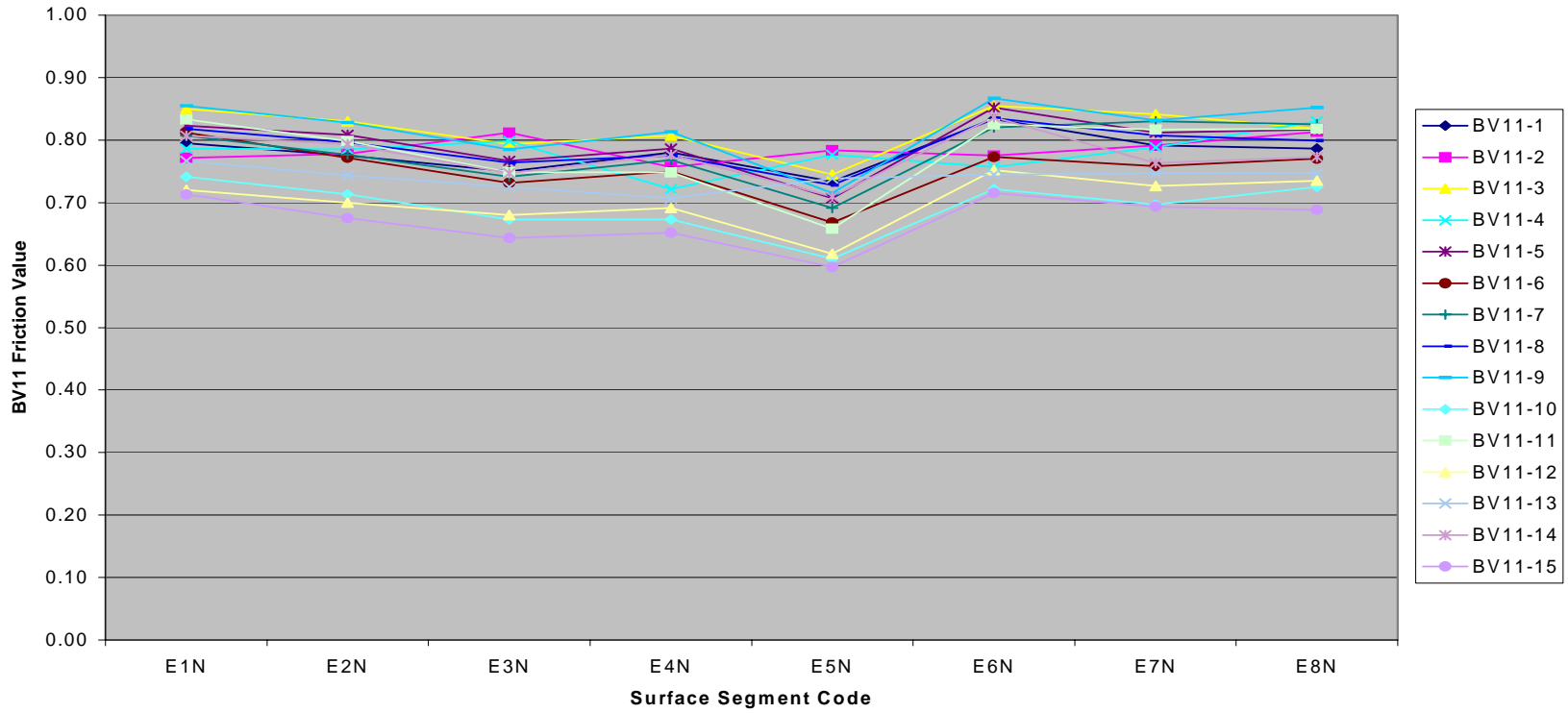
Figure 4. A sample extract of the NATAM database [8] for BV11 devices. Each friction value shown by marker is the average of three runs.
