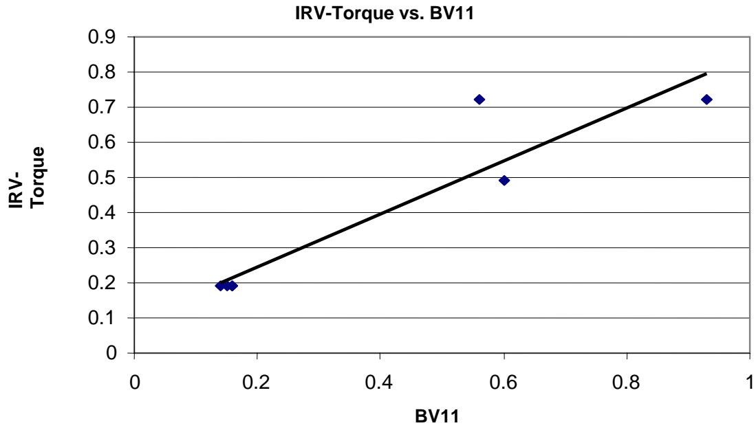
Figure 27. IRV Torque vs. BV11 – Operational Runs
