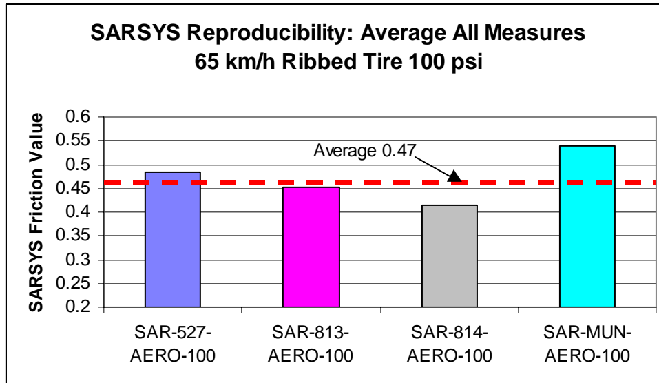
Figure 6. Average friction value of each device fitted with ribbed tires.
