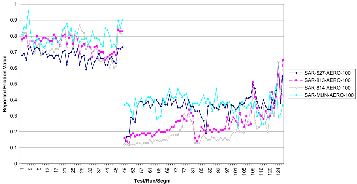
Figure 5. All reproduction data sets by run sequence at 65 km/h with ribbed tires inflated at 100 psi.
