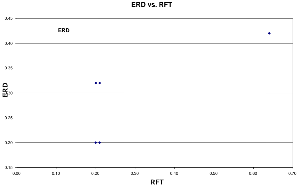
Figure 20. ERD vs. RFT – Operational Runs
