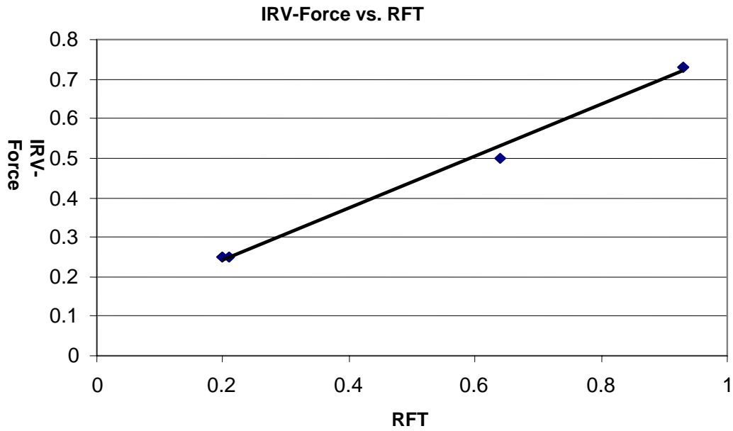
Figure 25. IRV Force vs. RFT – Operational Runs
