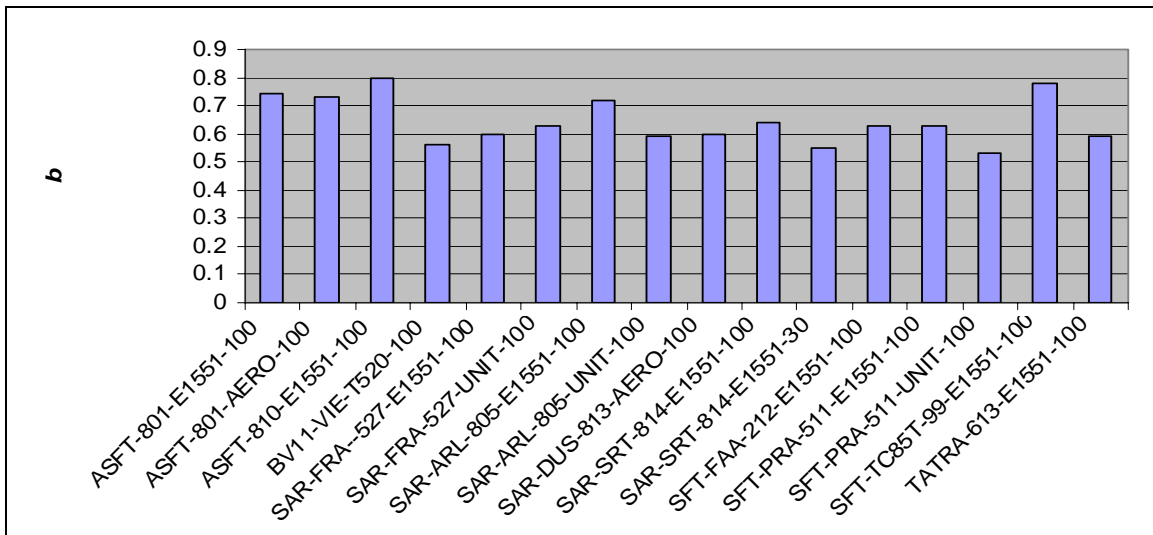
Figure 2 – 2002 Prague tests
