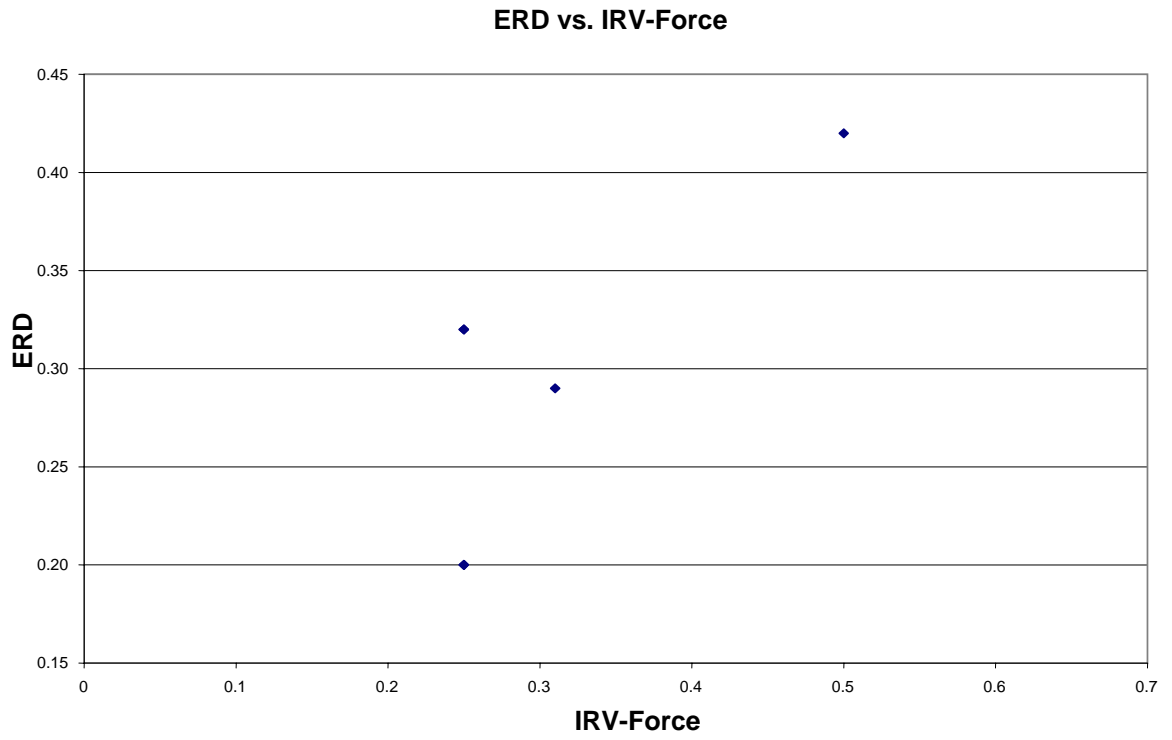
Figure 21. ERD vs. IRV Force – Operational Runs ERD vs. IRV-Torque
