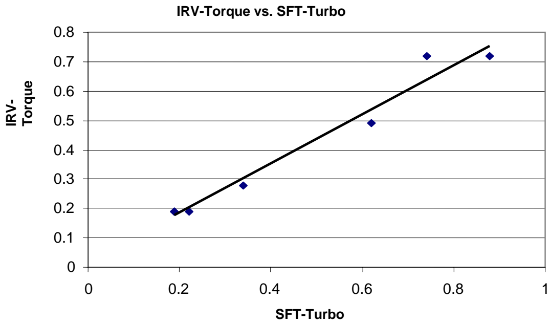
Figure 26. IRV Force vs. SFT-Turbo – Operational Runs
