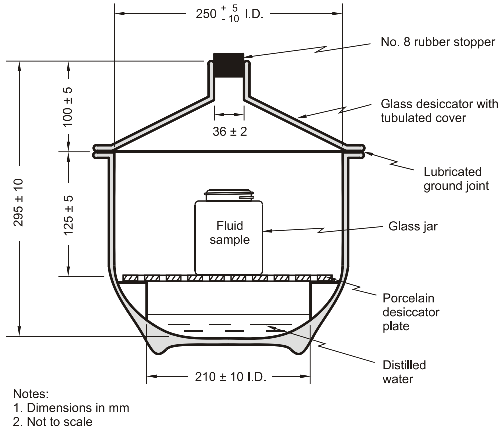
Figure 3 — Humidification Apparatus
