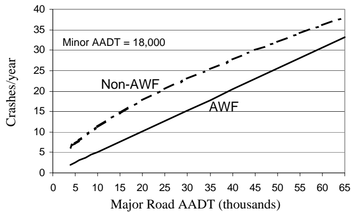
FIGURE 3.1: Advance Warning Flashers
