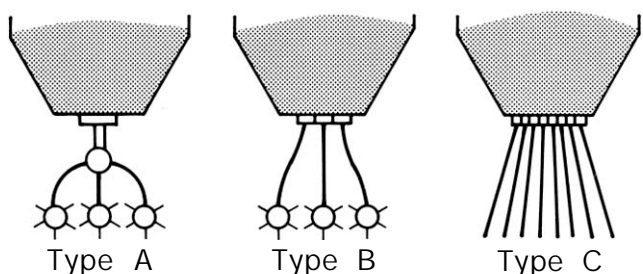
FIGURE 7. Air Seeder Distribution Systems.
