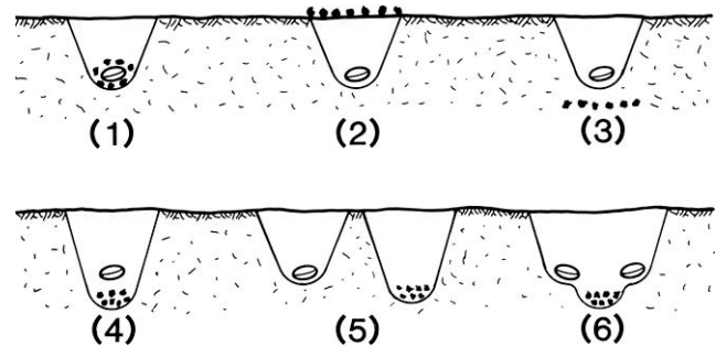
FIGURE 16. Fertilizer Placement: (1) Seed Placed, (2) Broadcast, (3) Pre-Seed Banded, (4) Below-Seed Banded, (5) Side Banded, (6) Paired Row Banded.
