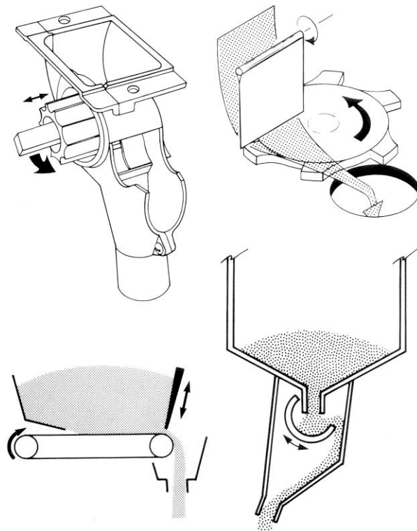
FIGURE 1. Variable Displacement Metering Mechanisms.
