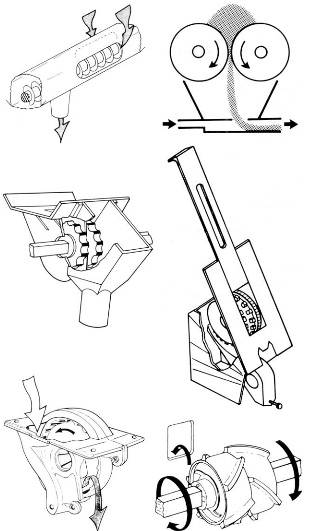
FIGURE 2. Variable Speed Metering Mechanisms.
