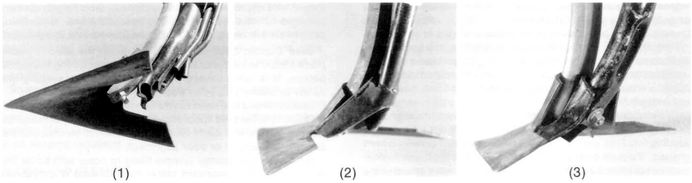
FIGURE 13. Air Seeder Boots: (1) Rearward Deflecting, (2) Forward Y-Dividing, (3) Forward Full Spreading.
