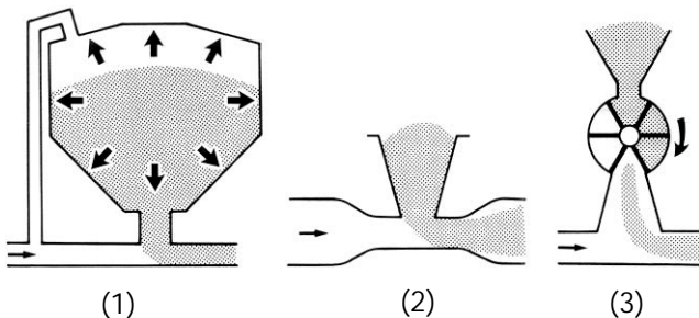
FIGURE 3. Airstream Loading on Air Seeders: (1) Pressurized Tank, (2) Venturi, (3) Air Lock Valve.
