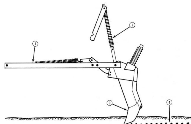
FIGURE 8 . Seed Placement Opener: (1) Frame, (2) Pressure and Depth Adjustment, (3) Soil Tool, (4) Seed and Fertilizer.
