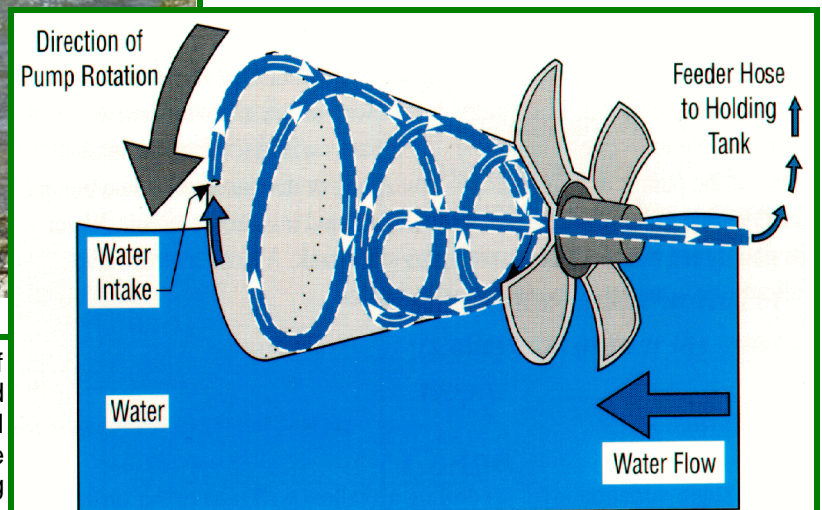
Sling Pump - Schematic
