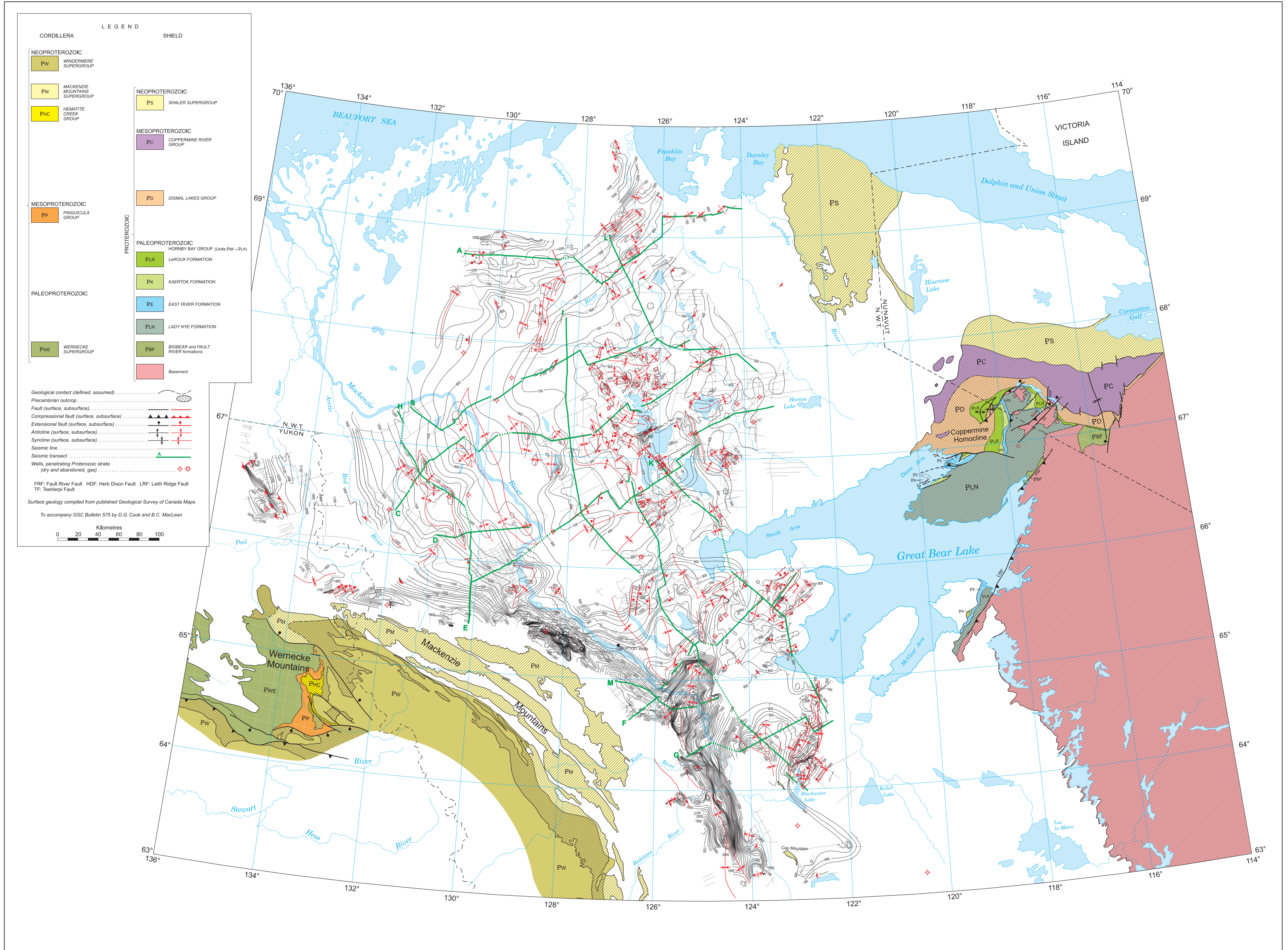
Figure 8. Seismic time-structure map of the sub-Cambrian unconformity. Contour interval is 50 ms two-way time. Modified from MacLean (1999).
