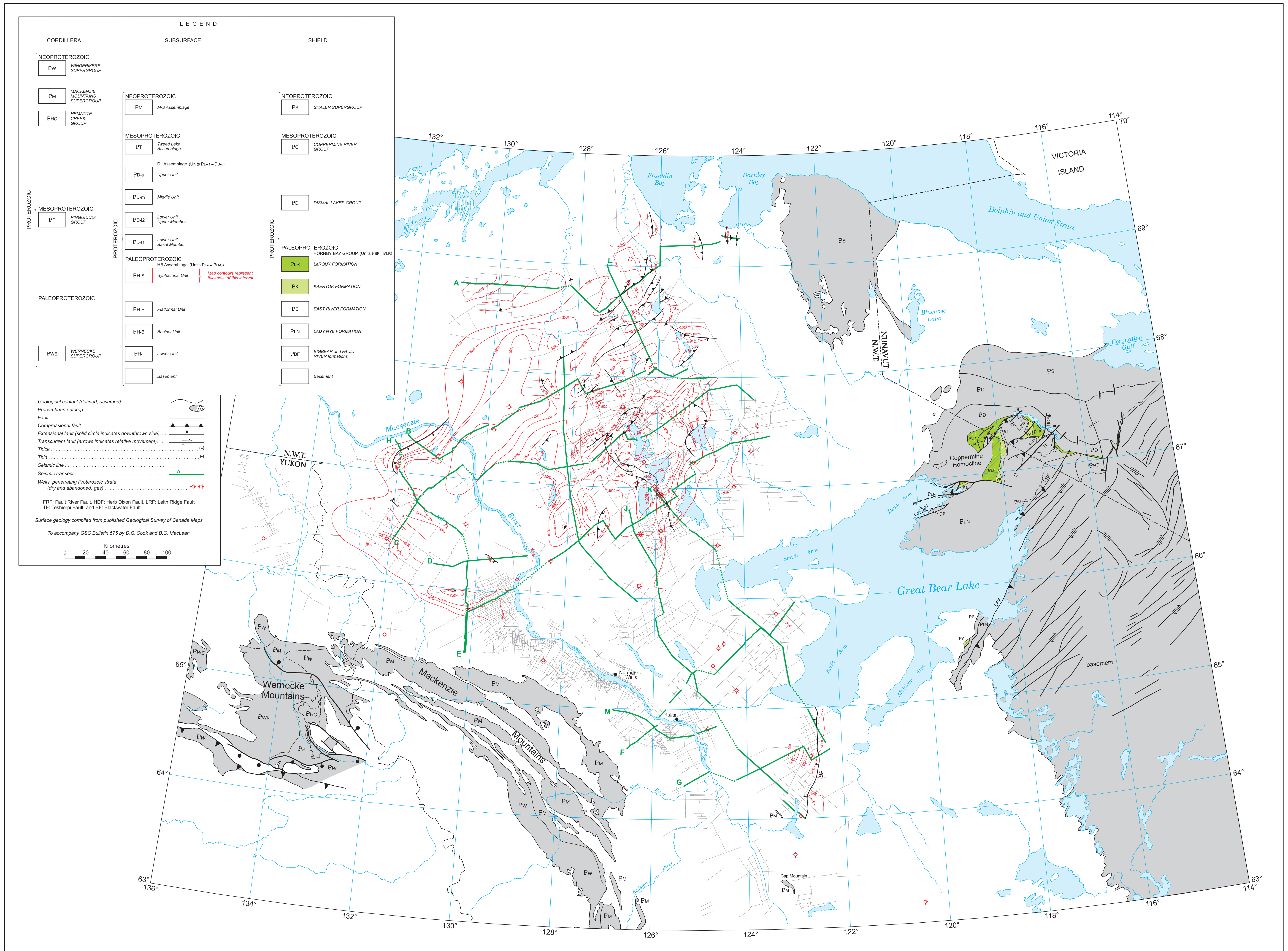
Figure 33. Thickness map of the Syntectonic Unit of the HB Assemblage, assuming a seismic interval velocity of 5800 m/s. Contour interval is 1000 m. Fault pattern within basement outcrop area is after Hoffman (1984) and St-Onge et al. (1991).
