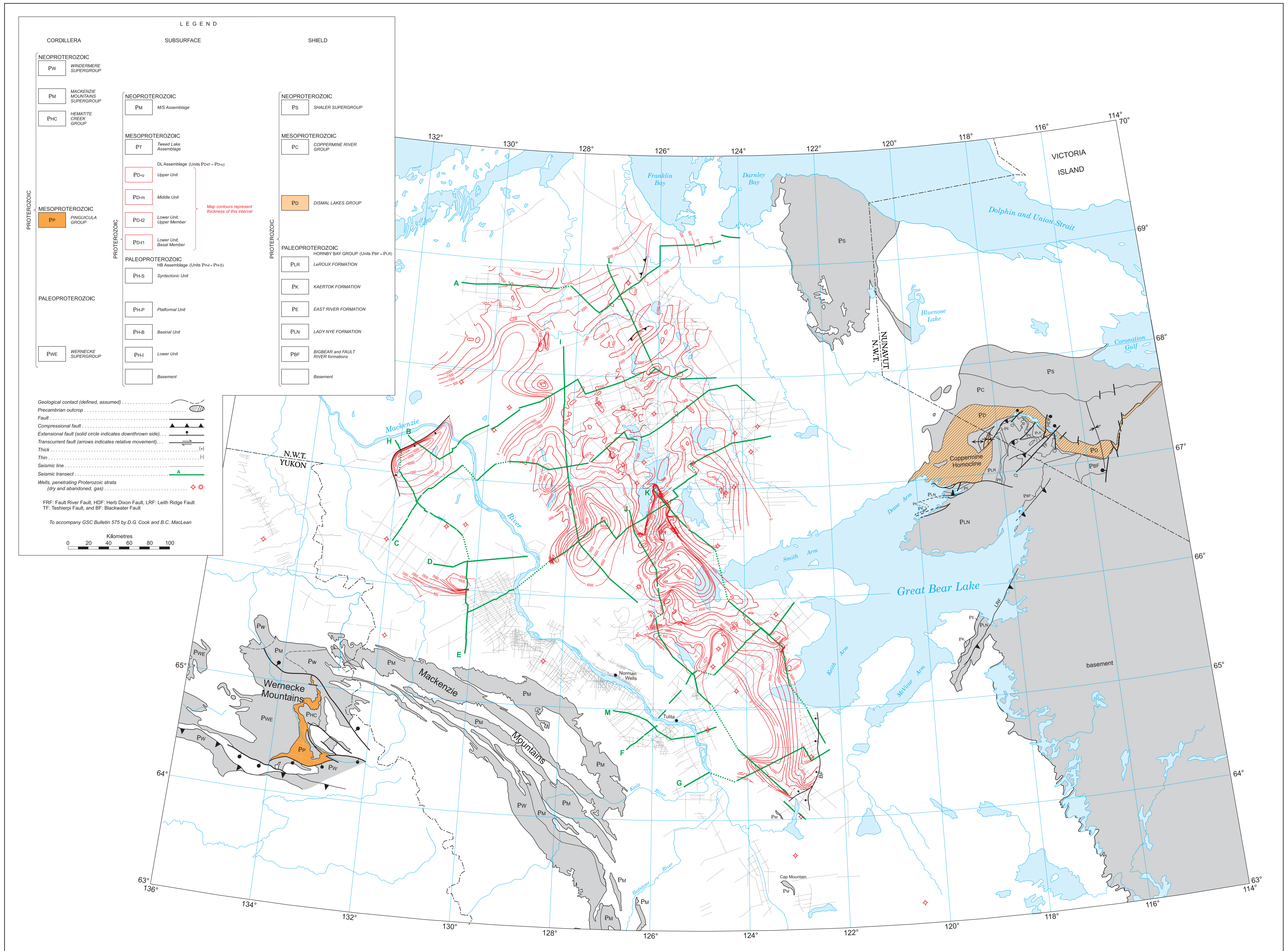
Figure 42. Thickness map of the DL Assemblage assuming a seismic interval velocity of 5400 m/s. Contour interval is 500 m.
