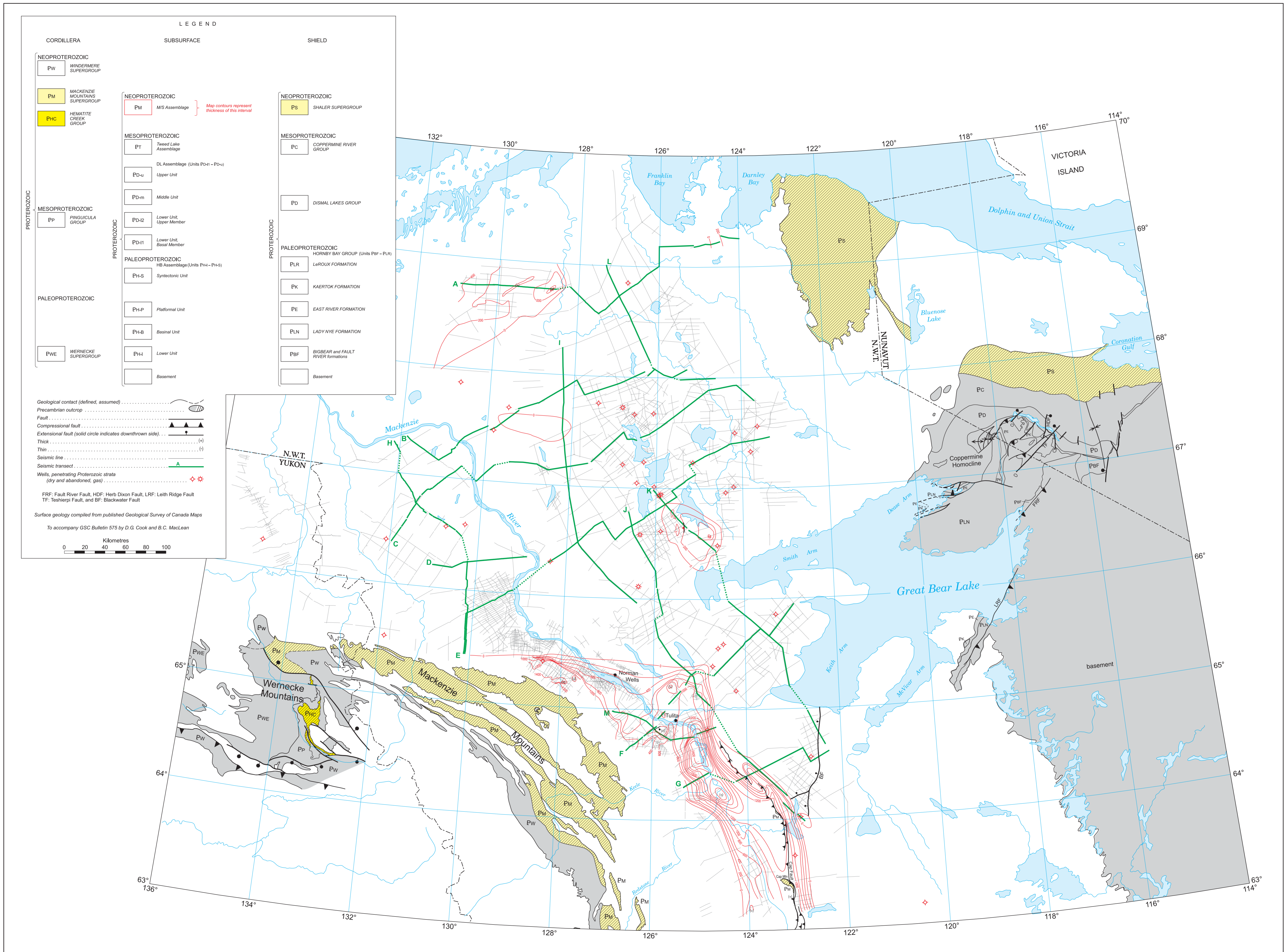
Figure 52. Seismic time-thickness map of the M/S Assemblage. Contour interval is 200 ms two-way time.
