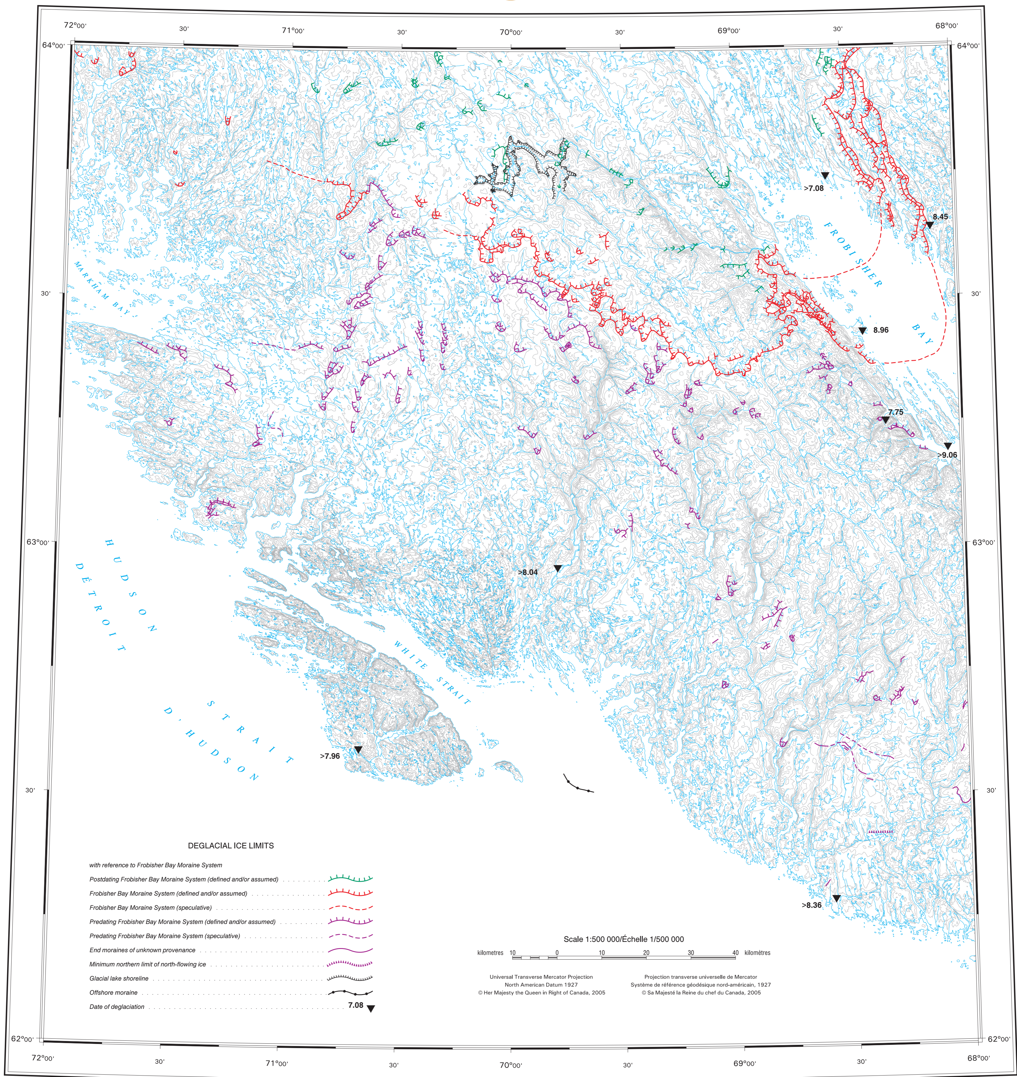
Figure 29. Ice margins during deglaciation (derived from moraine and meltwater drainage channel data).
