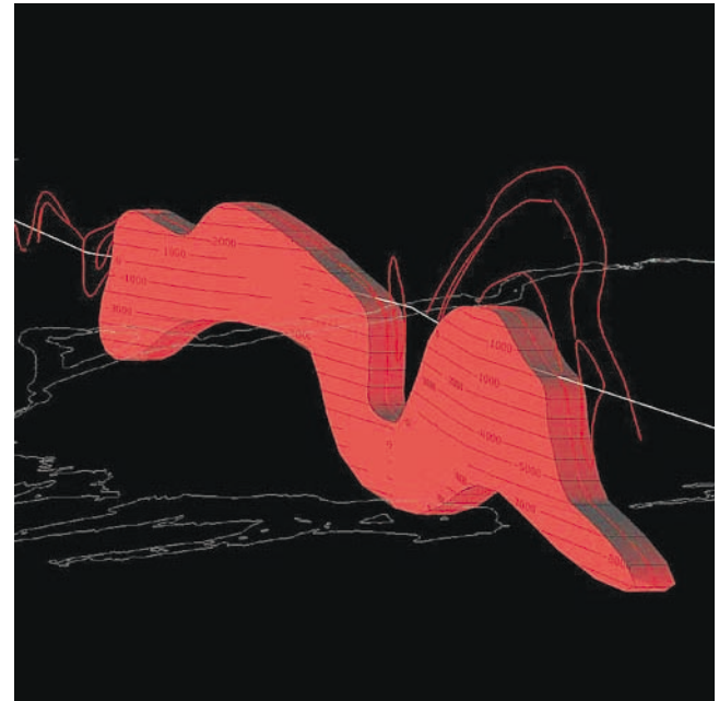
Figure 3. Perspective view of preliminary subsurface interpretation along section line depicted in Figure 2. Perspective view looking east-northeast.
