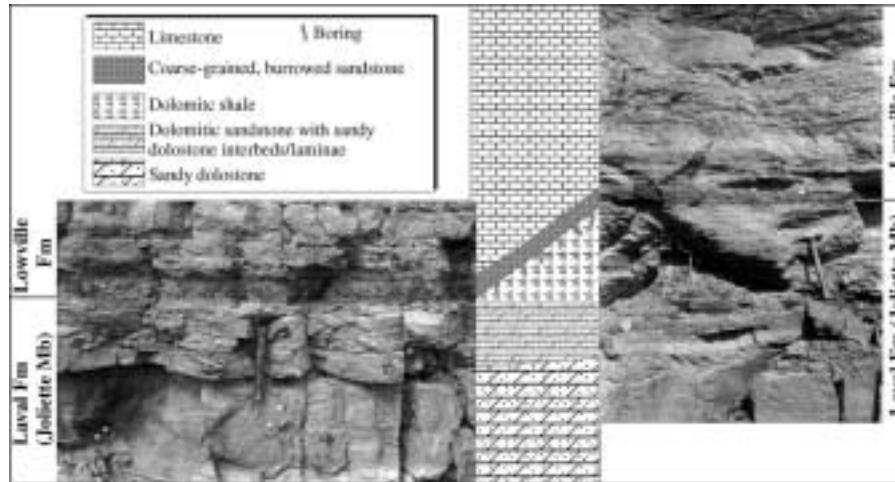
Figure 5. Correlation of two field pictures from the same quarry (St. Laurent cement quarry at Joliette, Quebec). Note that the thick dolomitic shale beds at top of the Laval Formation (here Joliette Member) present in the photograph at the right side of the figure is missing in the one to the left. The top of the dolomitic shale is bored (see Fig. 6) and overlain by coarse-grained, burrowed sandstone attributed to the overlying Lowville Formation. Here lithology assignable to the Pamela Formation is missing. This truncation of the upper Laval beds and borings suggest uplifting of the region, and also that the Laval Formation was indurated prior to the deposition of the Lowville Formation. A distance of about 60 m separates areas from which the two photographs were taken.
