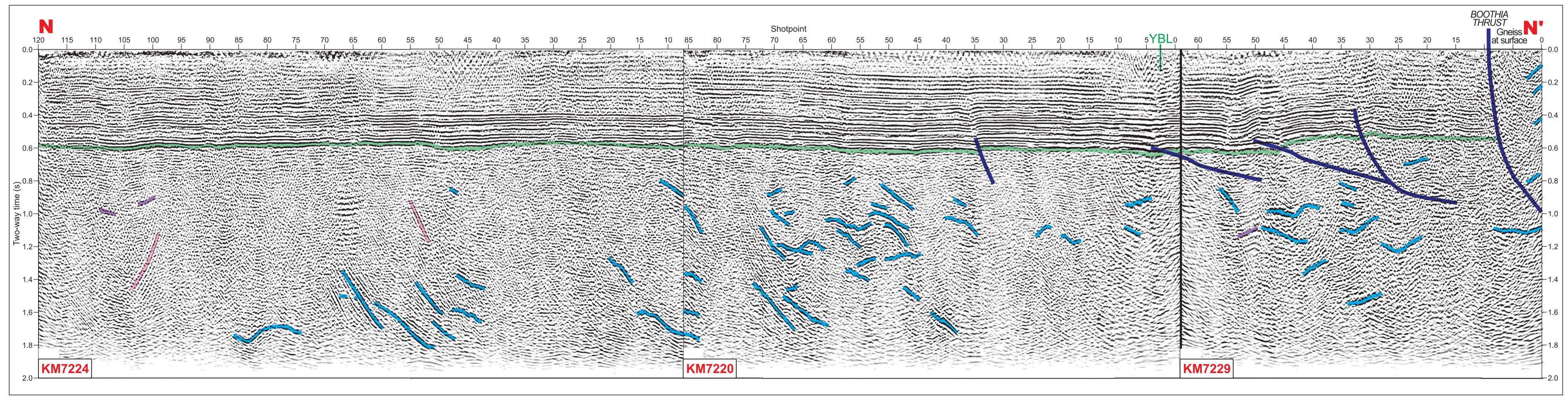
Figure 19. Seismic basement structure cross-sections.
