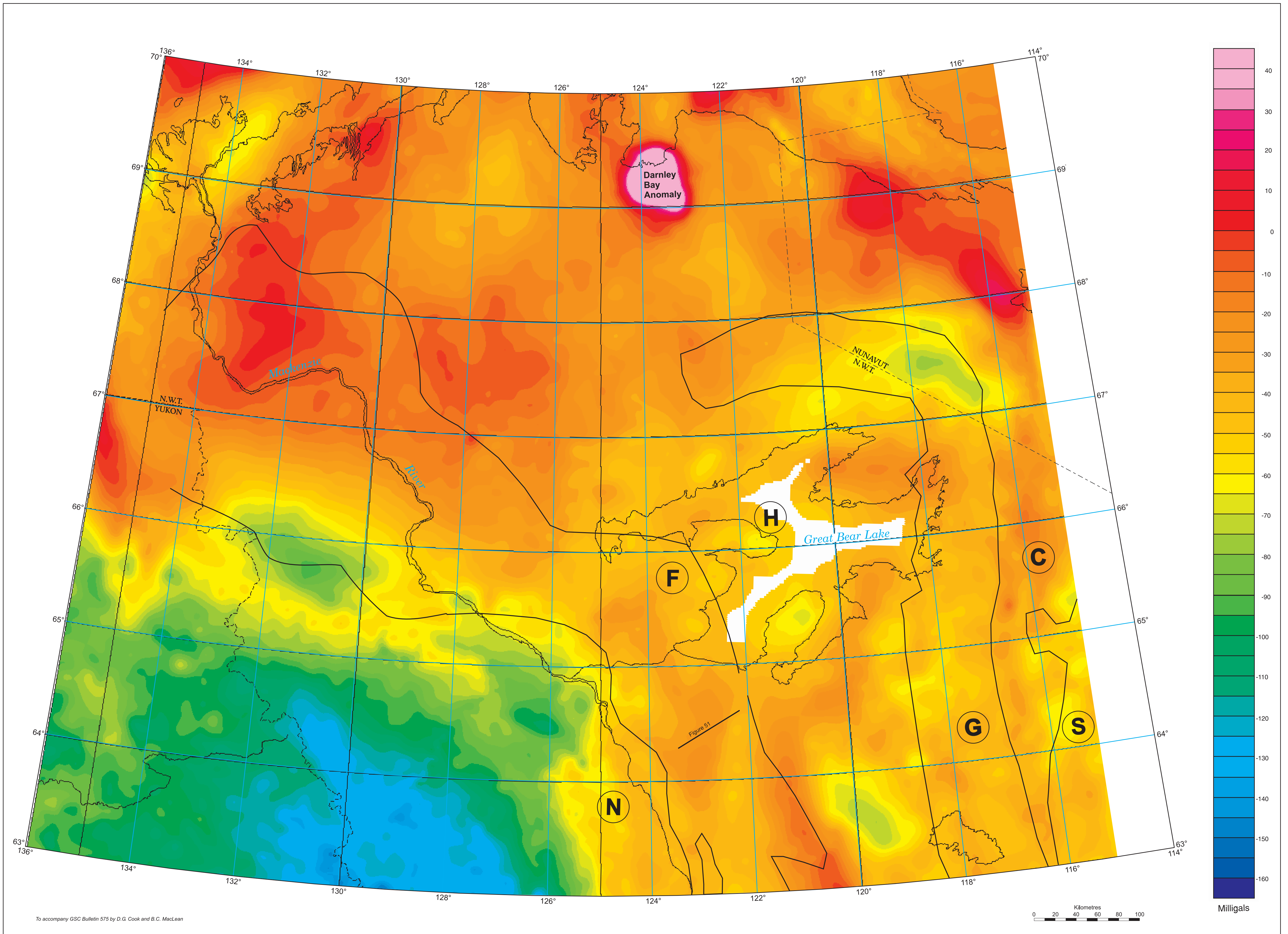
Figure 6. Bouguer gravity anomaly map (free air offshore) (data from Continental Geoscience Division, Geological Survey of Canada). Basement terrane boundaries and age limits are after Ross (1991). N, Nahanni (age unknown); F, Fort Simpson (1.79–2.02 Ga); H, Hottah (1.85–2.38 Ga); G, Great Bear (1.79–2.02 Ga); C, Coronation (1.85–2.38 Ga); S, Slave (2.6–3.9 Ga).
