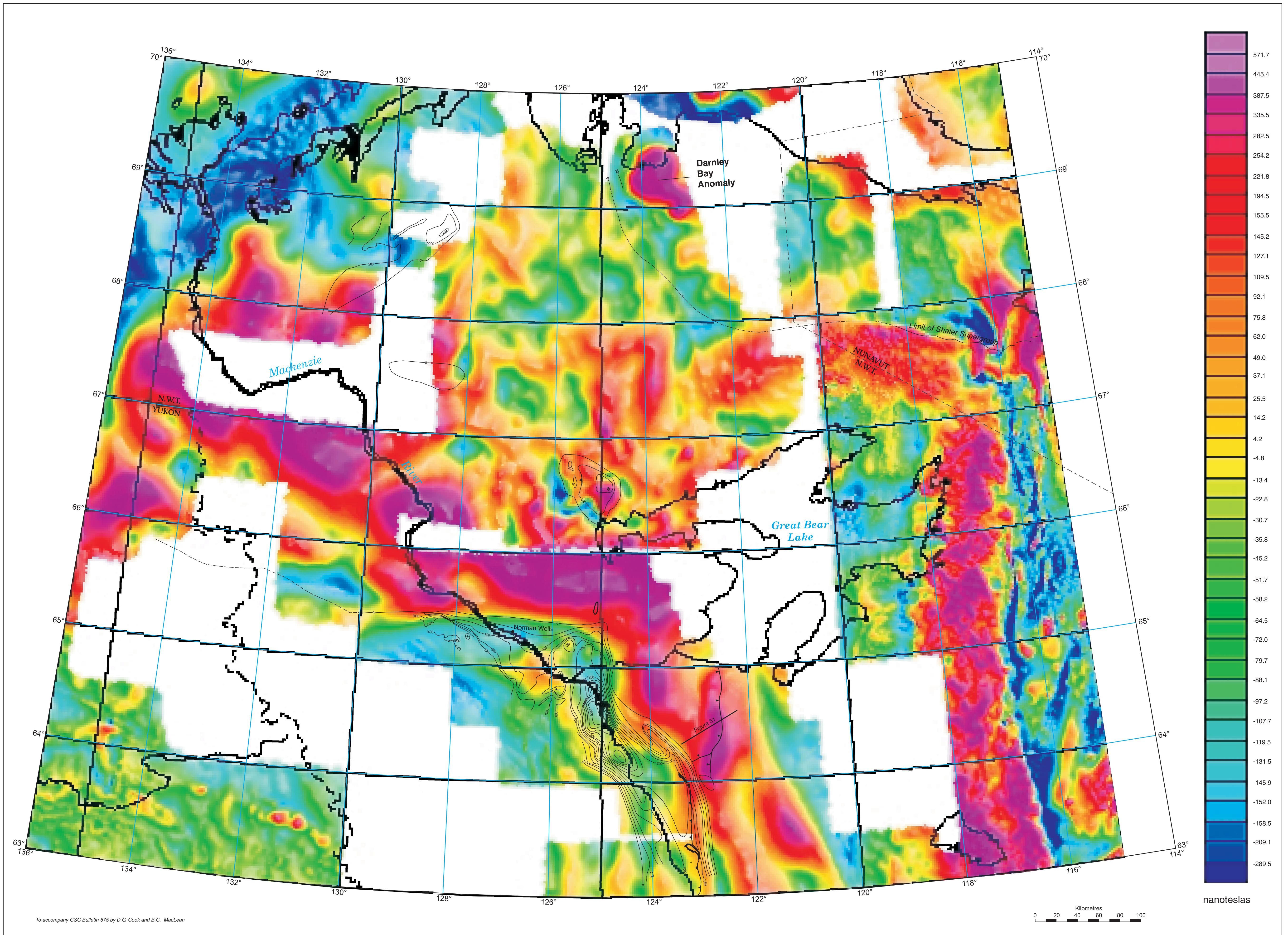
Figure 7. Total field aeromagnetic map with contours of the seismic time-thickness of M/S Assemblage overlain (indicating a general correspondence between M/S Assemblage and low magnetic values). Contour interval is 200 ms two-way time.
