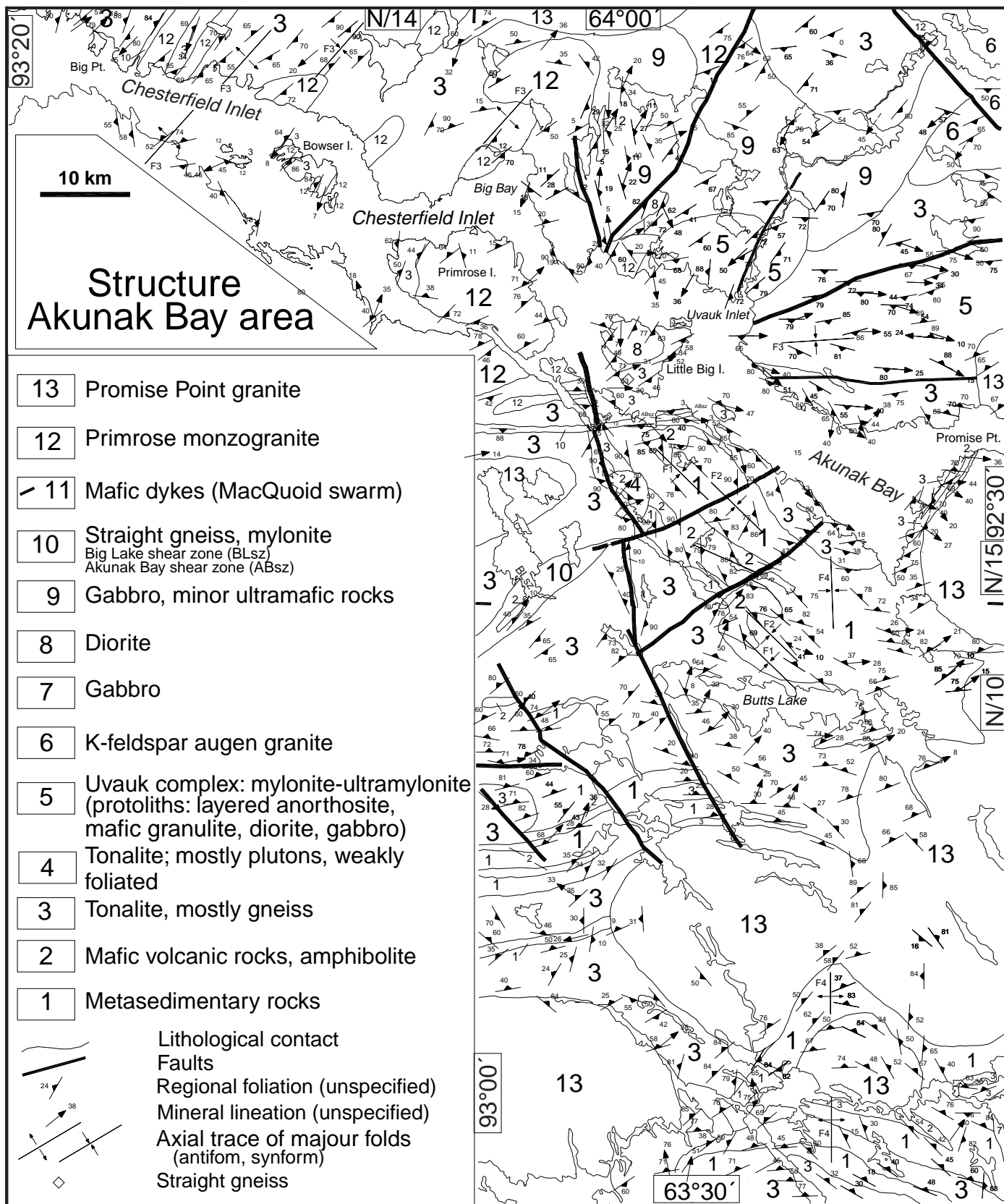
Figure 3. Simplified structural map of the Akunak Bay area (NTS 55 N).
