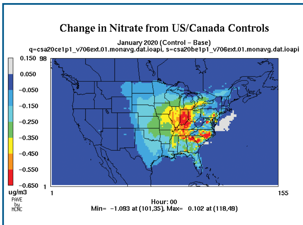
Figure 5.10b - Reductions in January \text{NO}_3 concentrations from controls in 2020.
