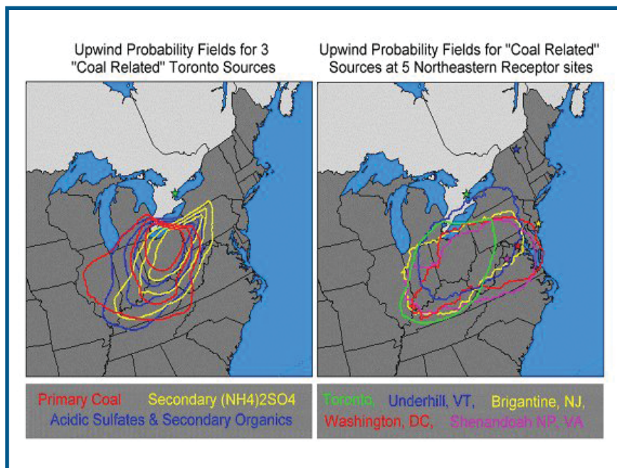
Figure 6.14 - Incremental probability fields for coal-related sources at Toronto and other eastern sites.
