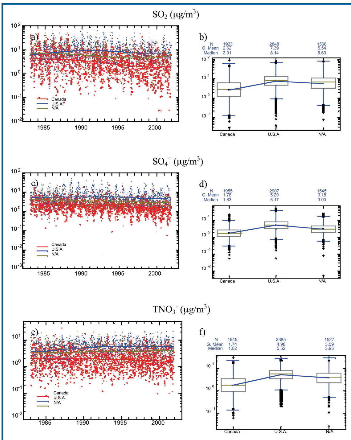
Figure 6.5 - Long-term trends and median concentrations of \text{SO}_2 (a and b, respectively), particle \text{SO}_4^- (c and d, respectively) and particle \text{NO}_3^- (e and f, respectively) in air at Longwoods, Ontario associated with three-day back trajectories from Canada, the United States and “Not Attributable” (N/A) to either sector. The trend line in the box plots connects the geometric means, the line dividing the boxes represents the median, the upper and lower sides of the boxes represent the 75th and 25th percentile of the data, respectively and the upper and lower bars on the box plots represent the 75th percentile plus 1.5 times the inter-quartile range and the 25th percentile minus 1.5 times the inter-quartile range, respectively.
