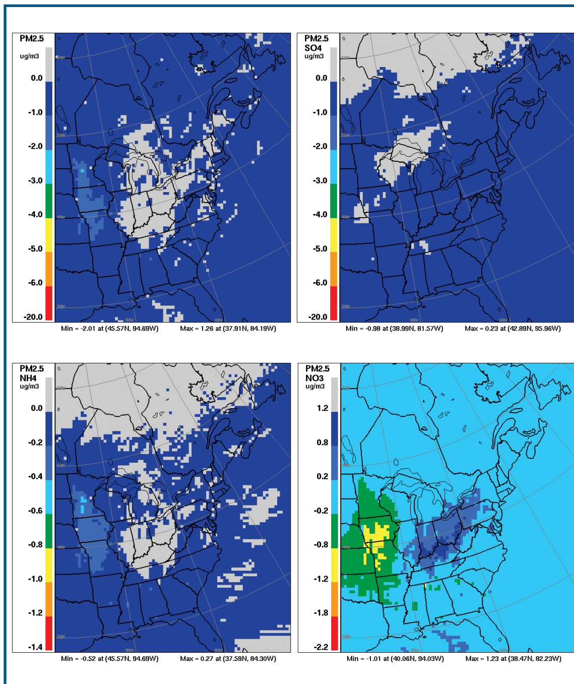
Figure 5.17 - Nine-day-average PM 2.5 mass concentration difference field and PM 2.5 inorganic chemical component concentration difference fields predicted by AURAMS for the Feb. 7-15, 1998 winter period for the “2010 control” case minus the “2010 base” case: (a) top left panel - PM 2.5 mass; (b) top right panel - PM 2.5 SO 4 mass; (c) lower left panel - PM 2.5 NH 4 mass; (d) lower right panel - PM 2.5 NO 3 mass. All fields are at 15 m height in units of µg/m 3 . Negative values denote a reduction for the “2010 control” case relative to the “2010 base” case.
