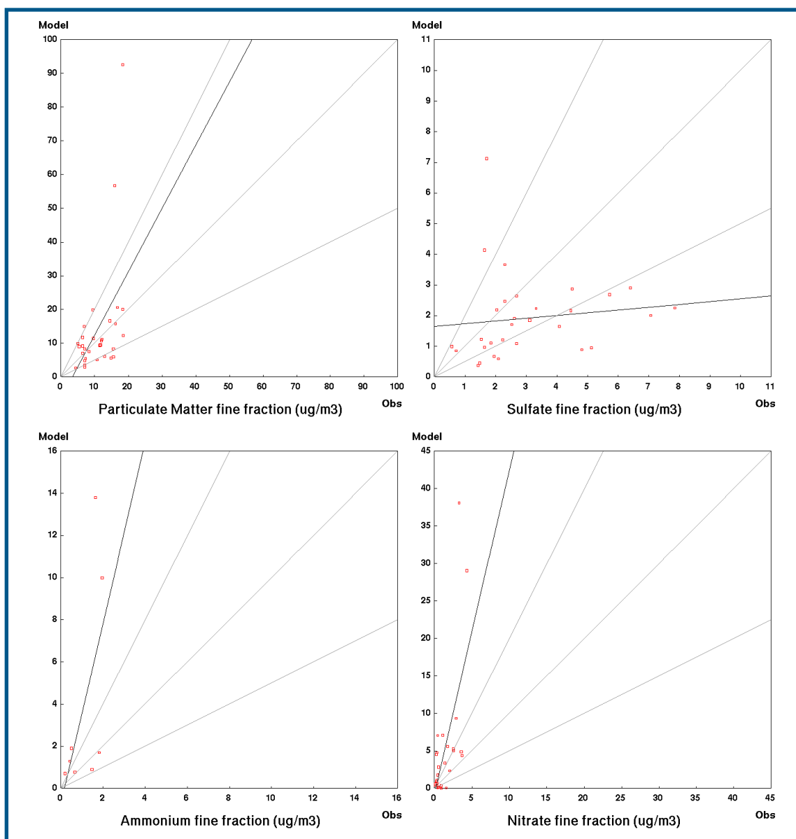
Figure A.5 - Scatter plots of daily (a) PM_{2.5} mass, (b) PM_{2.5} SO_4^- , (c) PM_{2.5} NH_4^+ , and (d) PM_{2.5} NO_3^- concentrations at all available IMPROVE and GAViM stations over the AURAMS domain for all days from February 7th 00Z to 14th 00Z 1998. Units are \mu g/m^3 at ambient conditions. The black line is a best-fit line and the gray lines are 2:1, 1:1 and 1:2 model-to-observation ratio lines.
