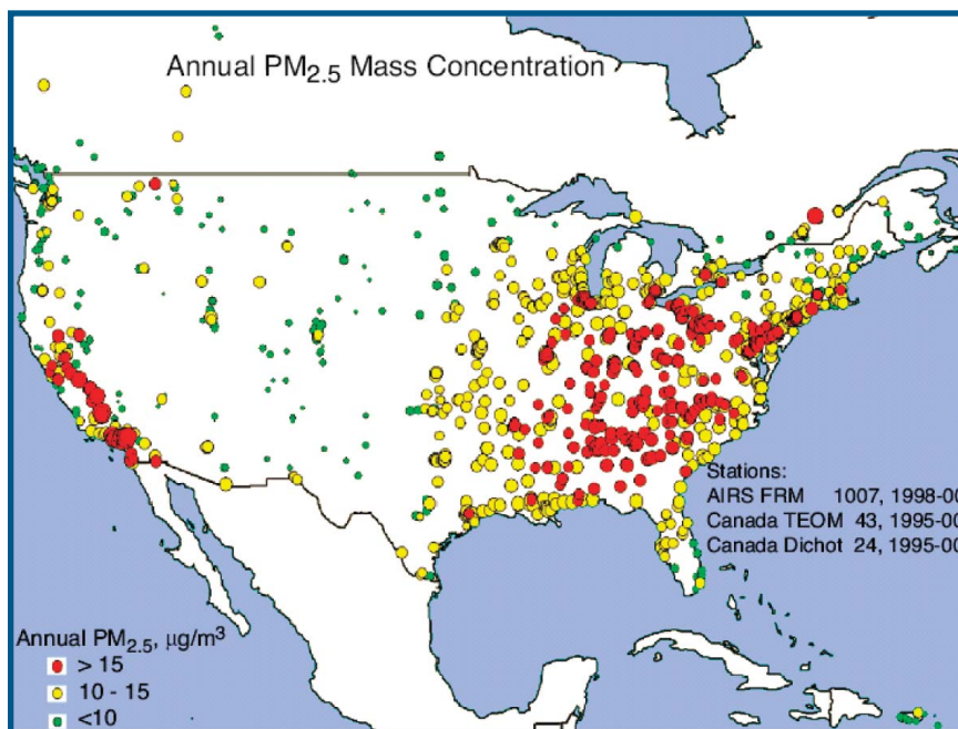
Figure 2.1 - Average PM 2.5 concentrations. The U.S. data are from FRM monitors at sites in the EPA AIRS database for July 1998 through July 2000. Canadian data are from TEOM and dichotomous samplers operating from 1995 through 2000. The currently available data from sites in Mexico represented less than one year of sampling and were excluded from the computation of annual averages. Spot diameter varies in proportion to concentration.
