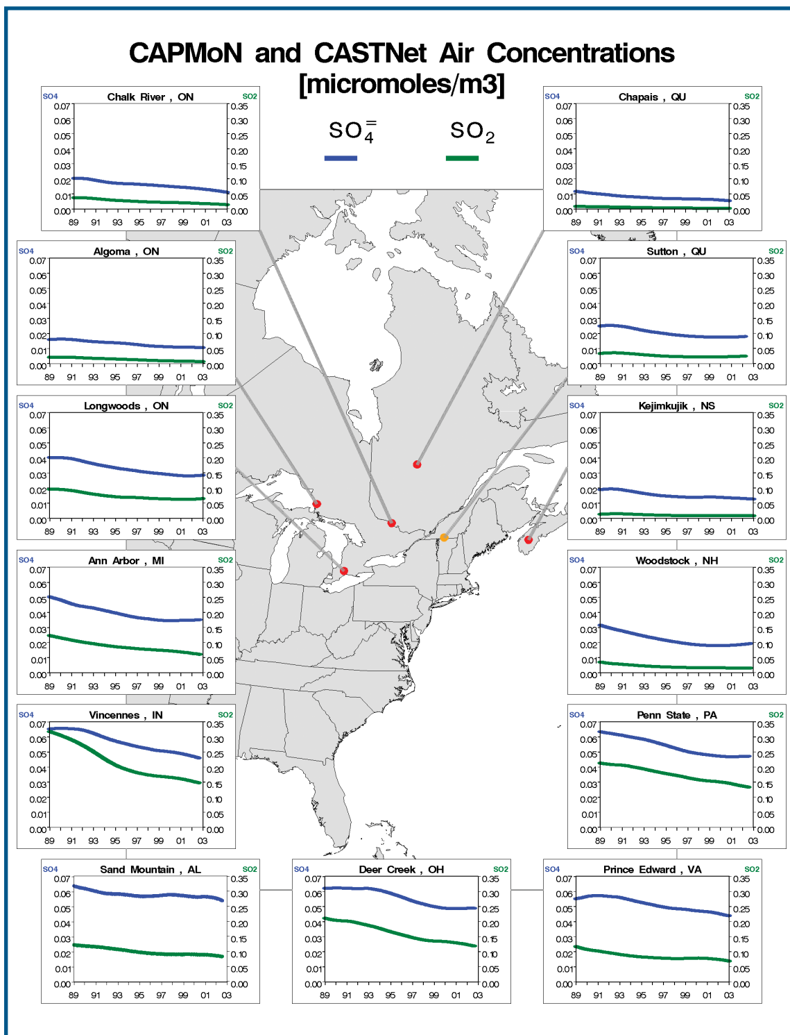
Figure 3.3 - Long-term trends in the precursor gases SO 2 (green) and particulate SO 4 - (blue) at rural CAPMoN and CASTNet sites, 1989–2002.
