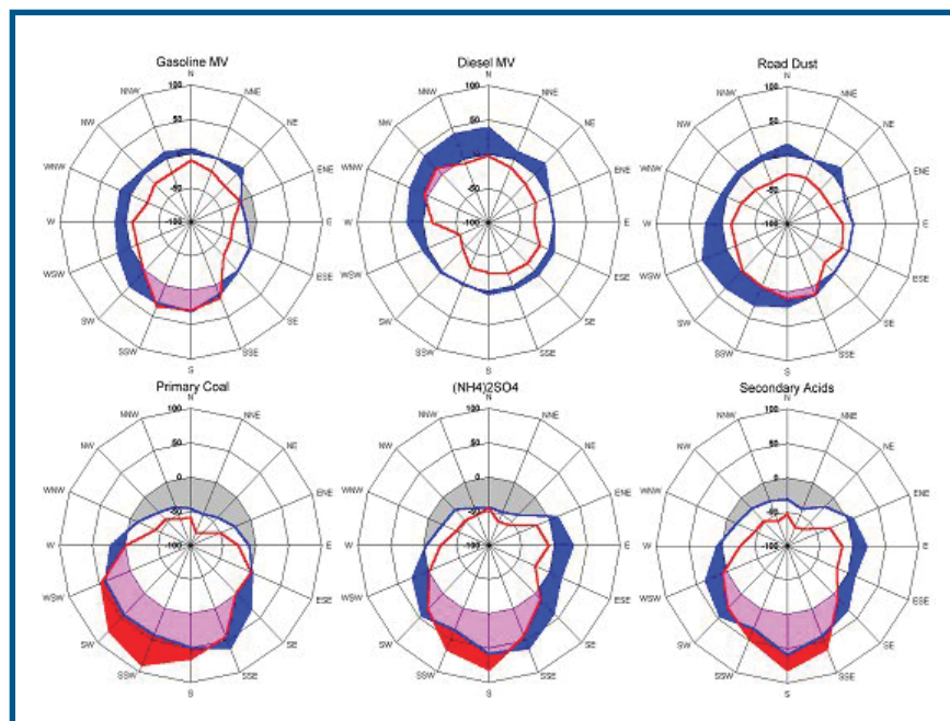
Figure 6.13 - UNMIX motor vehicle and coal-related sources vs. local surface wind speed and direction. Blue shading emphasizes directions from which source influence is greatest at low wind speeds. Pink shading emphasizes directions where source influence increases at all wind speeds. Red shading emphasizes directions from which source influence increases at high wind speeds.
