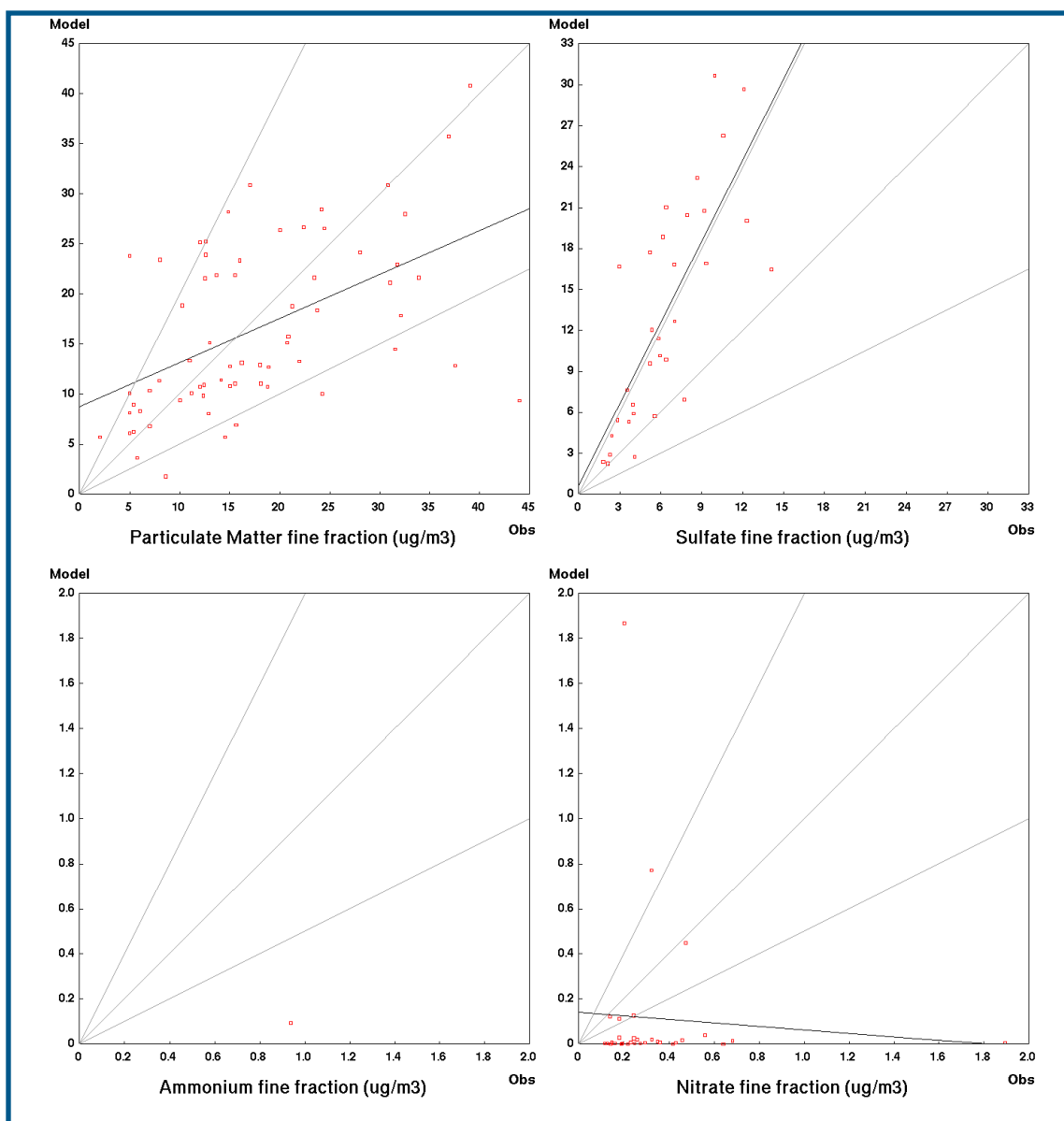
Figure A.10 - Scatterplots of daily (a) PM 2.5 mass, (b) PM 2.5 SO 4 2- , (c) PM 2.5 NH 4 + , and (d) PM 2.5 NO 3 - concentrations at all available IMPROVE, GAViM and CAAMP stations over the AURAMS domain for all days from July 8th 00Z to July 16th 00Z, 1995. Units are \mu\text{g}/\text{m}^3 at ambient conditions. The black line is a best-fit line and the gray lines are 2:1, 1:1 and 1:2 model-to-observation ratio lines.
