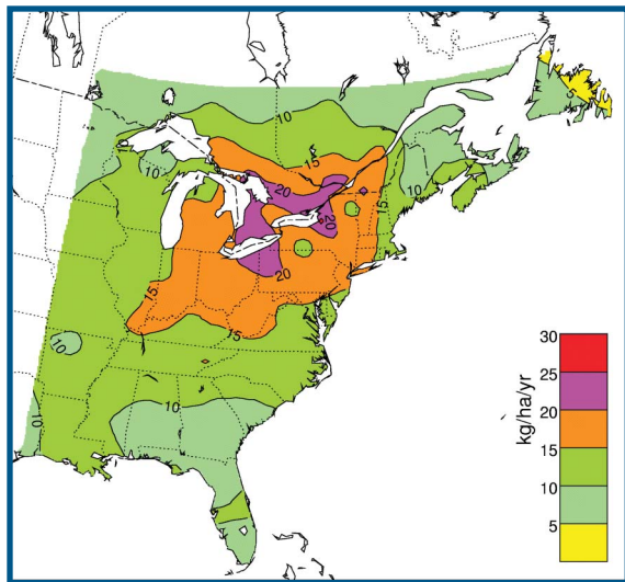
Figure 3.24 - Spatial distribution of wet \text{NO}_3^- deposition (kg/ha/yr) in eastern North America, 1996-2001.
