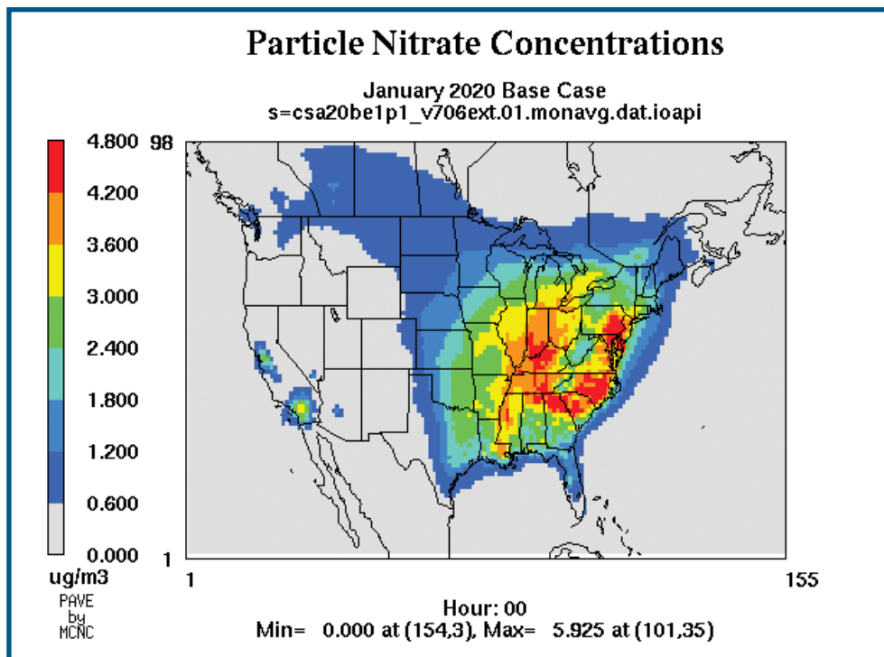
Figure 5.10a - January average \text{NO}_3 concentrations 2020 base case.
