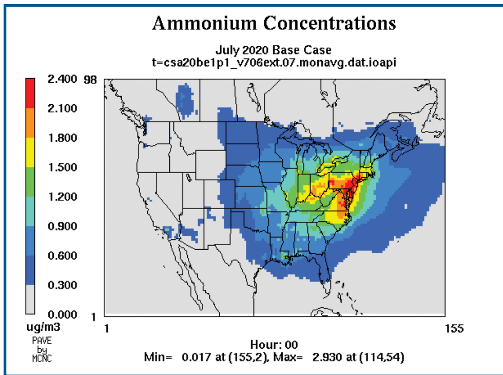
Figure 5.14a - July average \text{NH}_4^+ concentrations in 2020 base case.
