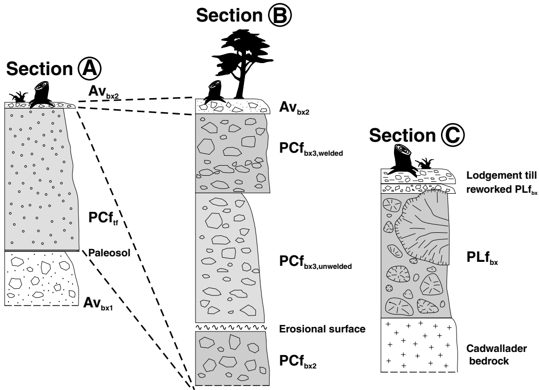
Figure 3. Schematic stratigraphic sections summarizing the distribution and stratigraphic relationships of major units of the Pebble Creek Formation. Locations are keyed to the geological map (Fig. 2) by letters: A) western limit of the Plinth avalanche overlying pyroclastic fall, B) eastern toe of the Plinth avalanche overlying late Pebble Creek block-and-ash flows, C) Plinth block-and-ash outlier sitting on bedrock upslope and east of B). Unit names and codes are the same as in Figure 2 (see text). Shaded units are volcanic in origin.
