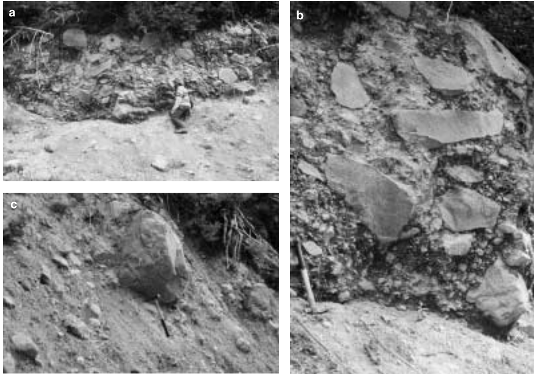
Figure 5. Field photographs of the block-and-ash avalanche deposit of the Pebble Creek Formation (Section B, Fig. 2) produced by the collapse of lava flows or domes. a) the deposit is variably welded and the photograph shows both an upper indurated facies and a lower unconsolidated facies. b) Close-up view of angular blocks within indurated facies of the Pebble Creek block-and-ash flow. There is little compaction of the blocks. c) An example of a delicate 'breadcrust'-textured block found within the poorly indurated facies of the Pebble Creek block-and-ash flow deposits. The hammer is 45 cm long.
