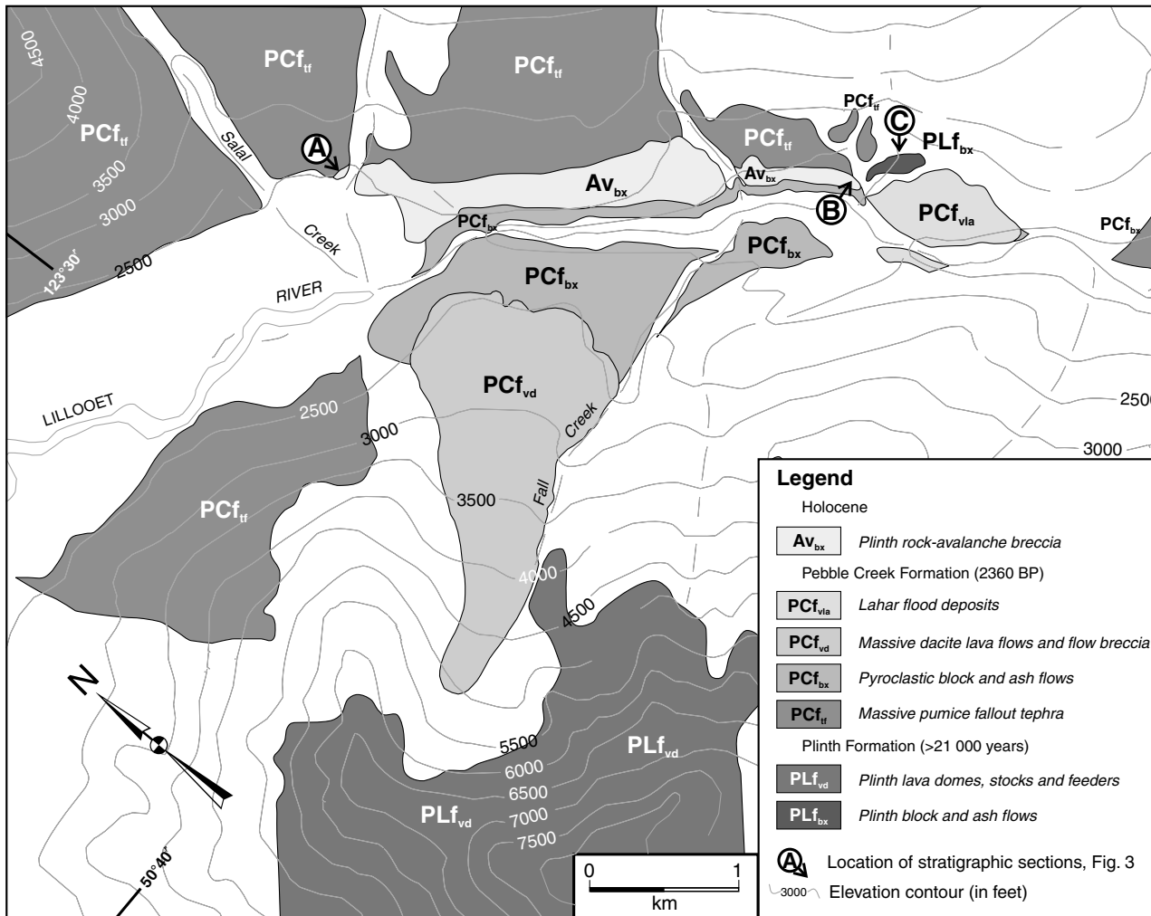
Figure 2. Geological map for the area situated immediately north of Mount Meager and along the Lillooet River. Stratigraphic units in the map legend include deposits of the Pebble Creek Formation defined by Hickson et al. (1999) and units identified or revised in this work. The locations of important stratigraphic sections discussed in the text are noted (see Fig. 3).
