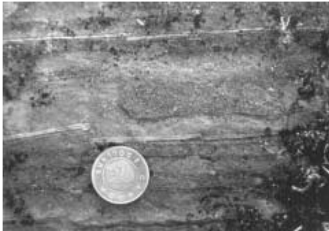
Figure 3. Millimetre- to centimetre-scale bedding in biotite psammite and semi-pelite. Note the small pebble-rich channel in the centre of the photograph. Two-dollar coin for scale.
