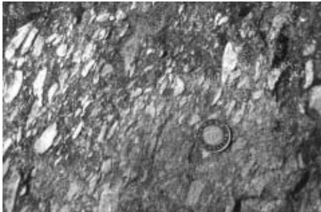
Figure 4. Matrix-supported poly-mictic conglomerate with subangular clasts of quartzite and felsic to intermediate volcanic rock in an intermediate-composition matrix (locality c on Fig. 2). Two-dollar coin for scale.
