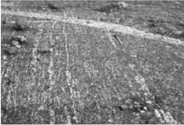
Figure 10. Metasedimentary diatexite or paragneiss of the Prince Albert Group comprising pinch and swell bands of muscovite+biotite granite (leucosome) with biotite+plagioclase±garnet±sillimanite melanosome. Note the crosscutting dyke of muscovite+biotite pegmatite. Hammer for scale is 1 m.
