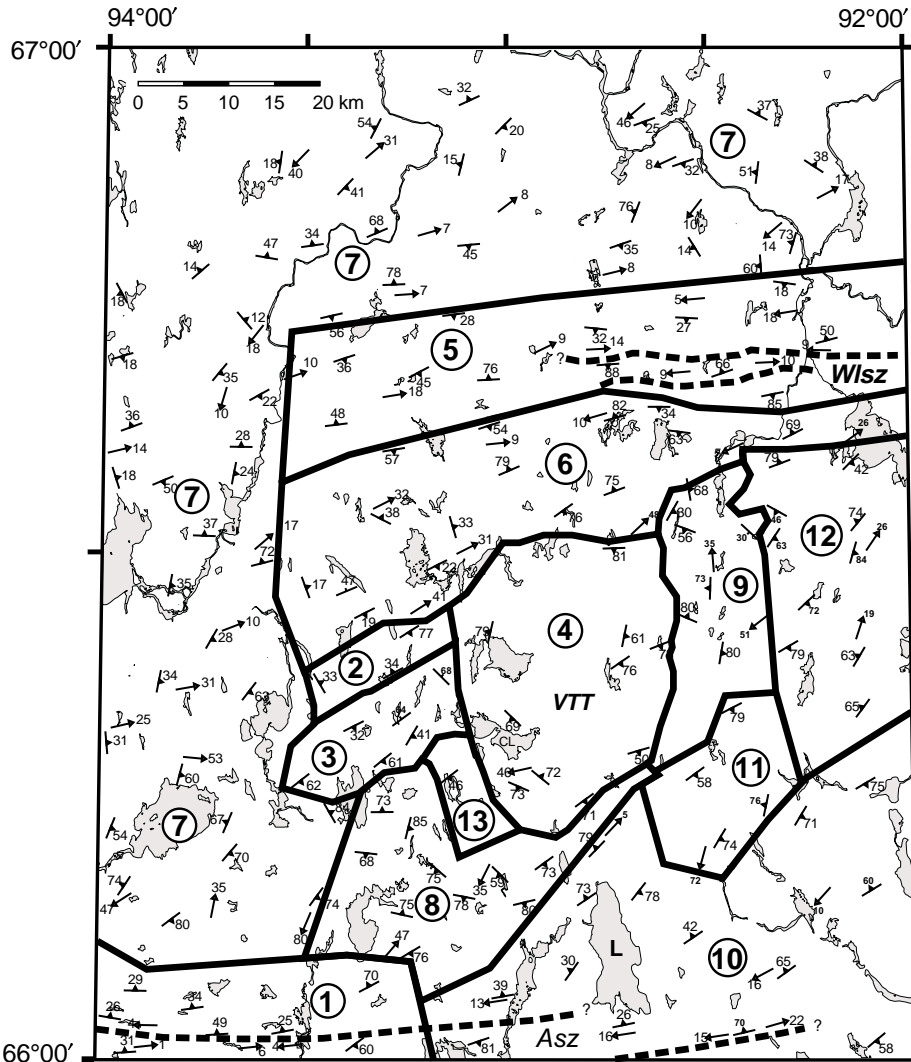
Figure 3. Simplified structural map of the Laughland Lake map sheet showing the distribution of structural domains discussed in the text. VTT = central tonalite, Asz = Amer shear zone, Wisz = Walker Lake shear zone.
