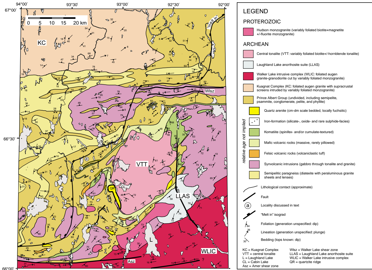
Figure 2. Generalized geology of the Laughland Lake map area. Letters are locations discussed in the text.
