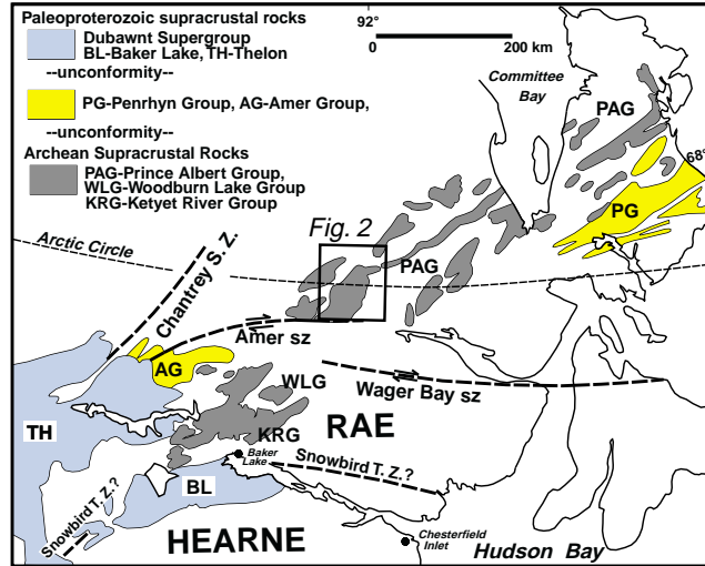
Figure 1. Regional geological setting of the study area northwest of Hudson Bay showing the distribution of Archean supracrustal rocks of the Prince Albert Group, the Woodburn Lake Group and the Ketyet River Group relative to the Paleoproterozoic supracrustal suites of the region. Adapted from Zaleski et al. (1997).
