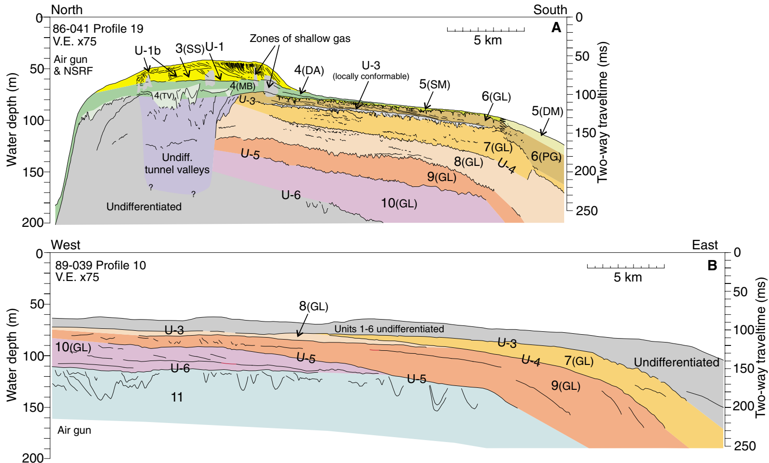
Figure 2. Geological sections compiled from NSRF V-fin and air-gun seismic profiles (locations, Fig. 1) illustrating the stratigraphic units and their bounding surfaces.
