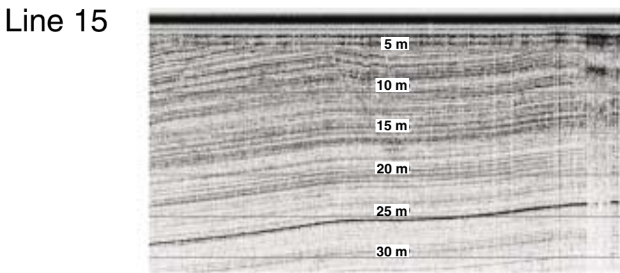
Figure 4. South-to-north profiles showing the rotated block of glaciomarine sediments. Vertical exaggeration is 5.5x.
