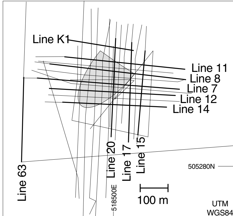
Figure 2. Track plot of the Chirp sonar survey area. Labelled, dark traces represent the profiles discussed in this paper. The thin traces show the extent of the coverage, but are not specifically discussed. The shaded area is the location of the rotated, disturbed zone.
