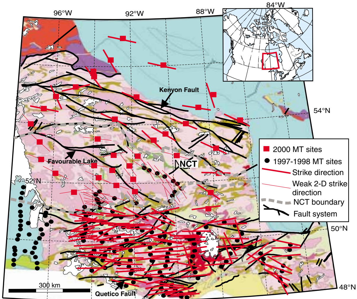
Figure 1. Site locations and 2-D strike directions. A weakly 2-D or approximately 1-D region falls within the boundaries of the North Caribou terrane (NCT).
