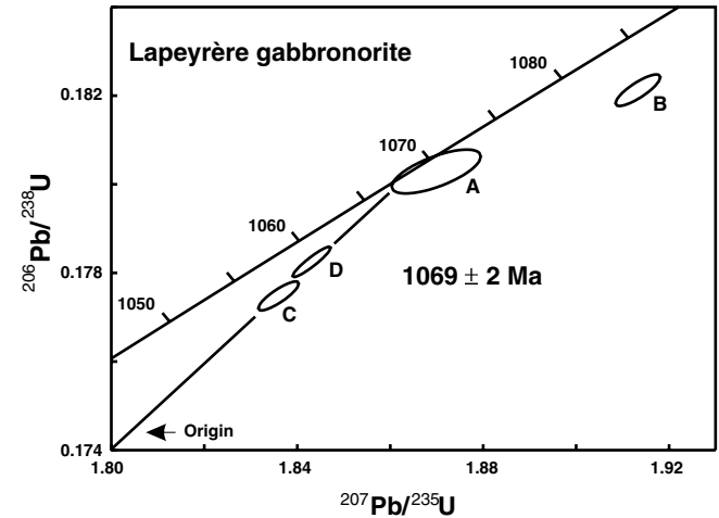
Figure 5. Concordia diagram of igneous zircon of the Lapeyrère gabbronorite. Error ellipses reflect the 2σ uncertainty.
