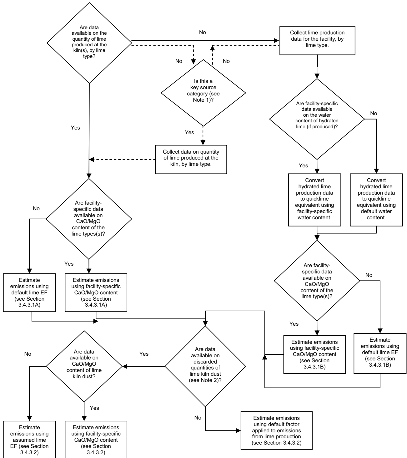
Figure 3: Decision Tree for Selecting the Method for Estimating CO 2 Emissions from Lime Production in the Kiln
