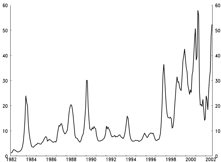
Figure 3: Weighted Average of Z-score, Big Six Banks*
