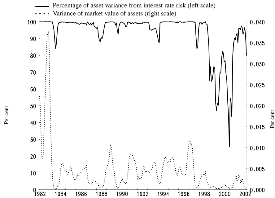
Figure 2: Big Six Banks: Decomposition of Asset Variance*
