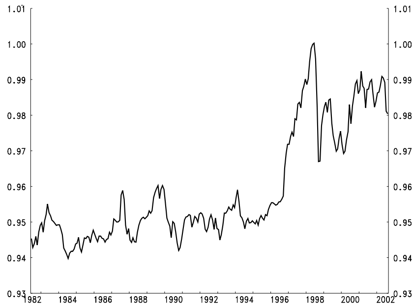
Figure 1: Weighted Average of Market-to-Book Ratio of Assets, Big Six Banks*
