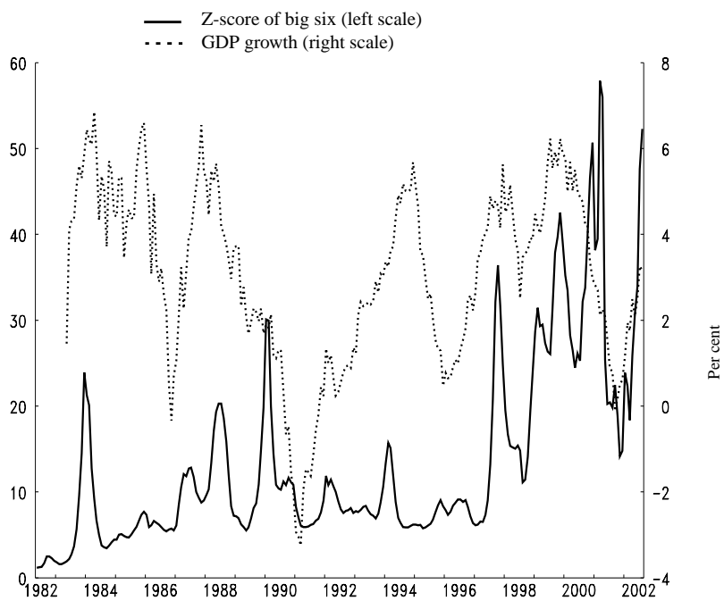
Figure 4: Z-score of Big Six vs. Output Growth
