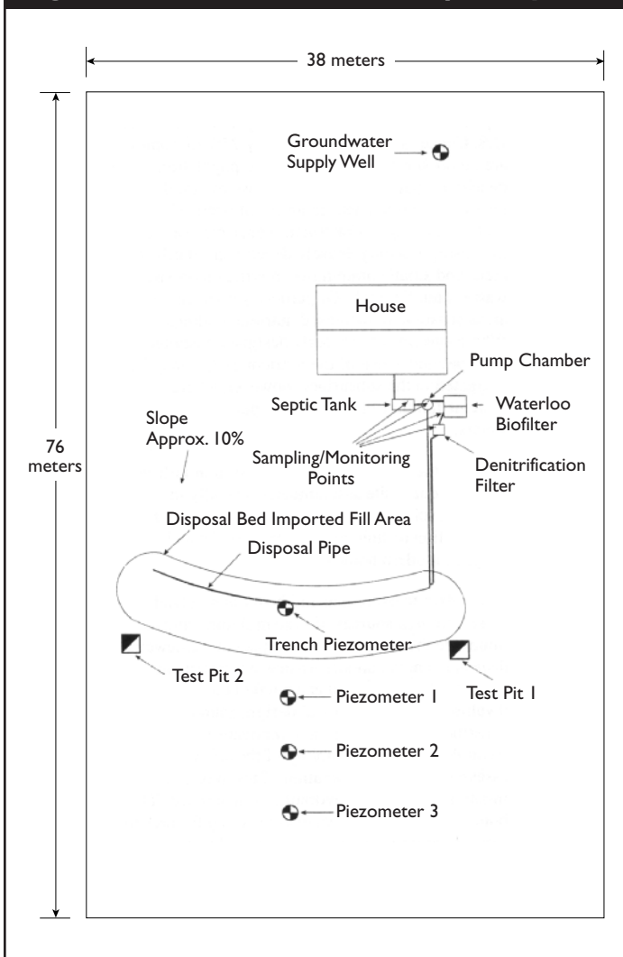
Figure 1: Plan view of lot and disposal system
