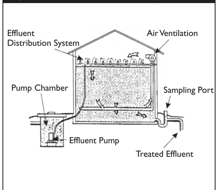
Figure 2: Waterloo biofilter configuration
