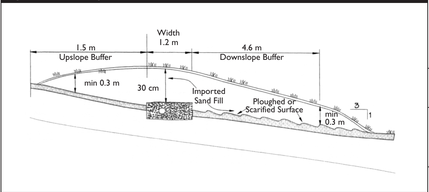
Figure 3: Contour disposal field cross-section
