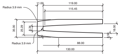
Figure 4a) - Basic brick tie
