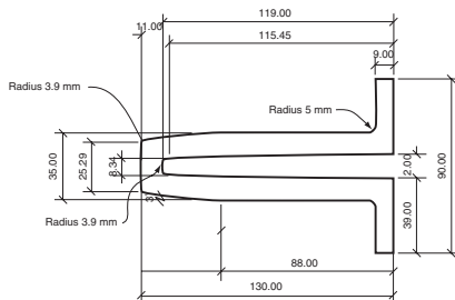
Figure 4b) - Brick tie with end returns
