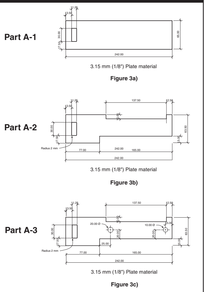
Figure 3: Basic block tie design and variations
