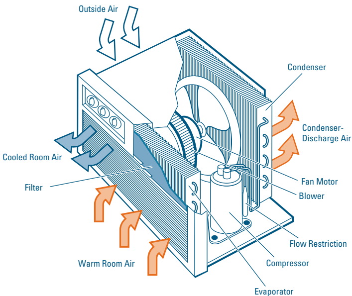
Figure 3 Components of a room air conditioner
