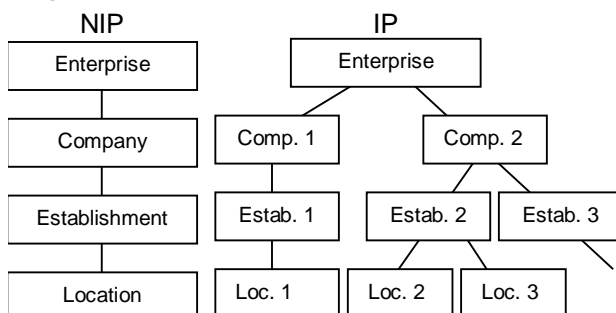
Diagram 2: Statistical Structures
