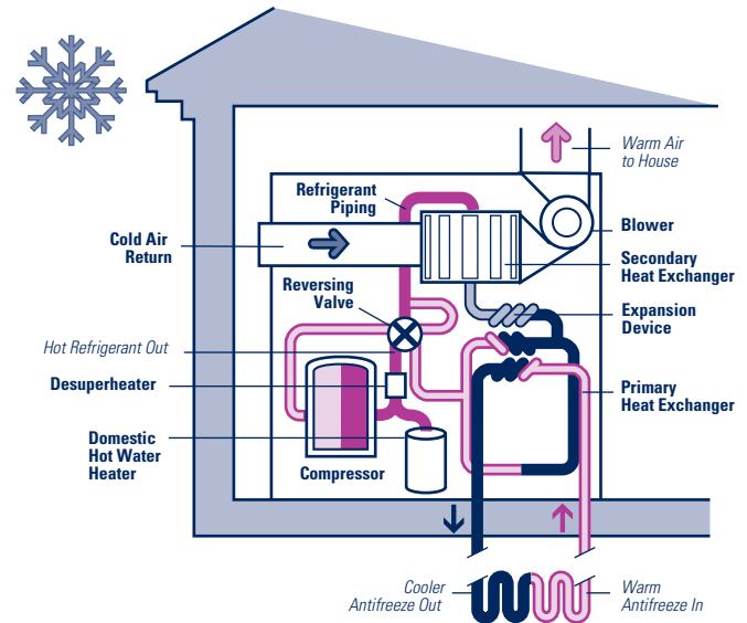
Figure 7: Components of a Typical Ground-Source Heat Pump
