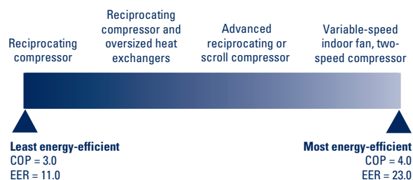
Figure 8: Open System Earth-Energy System Efficiency (at an entering water temperature of 10°C)
