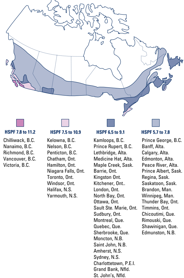
Figure 14: Heating Seasonal Performance Factors (HSPF) for Closed-Loop EES in Canada.
