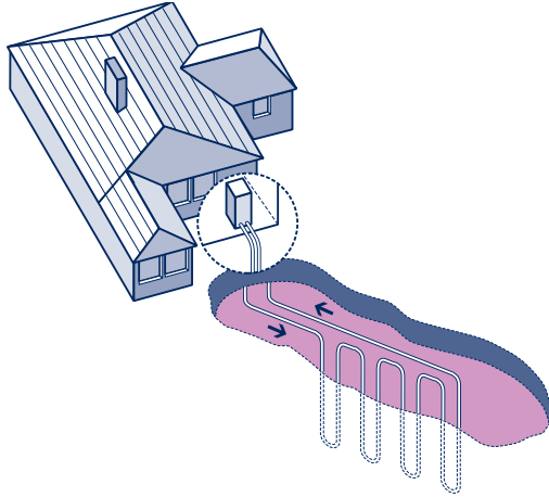
Figure 11: Closed-Loop, Single U-Bend Vertical Configuration
