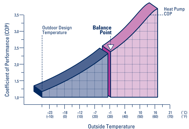
Figure 5: Performance Characteristics of a Typical Air-Source Heat Pump
