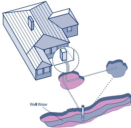
Figure 10: Open System Using Groundwater From a Well as a Heat Source
