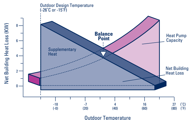
Figure 15: Balance Point for a Typical Air-Source Heat Pump
