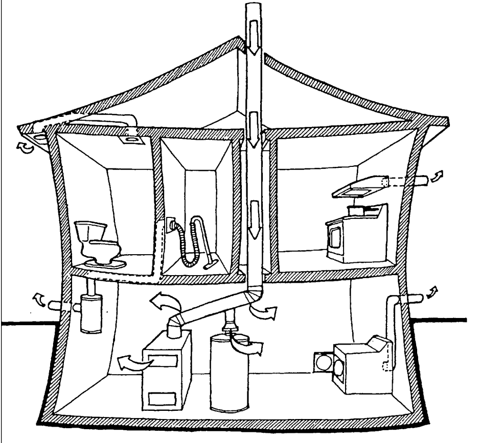
Figure 3: BACKDRAFTING DUE TO DEPRESSURIZATION
