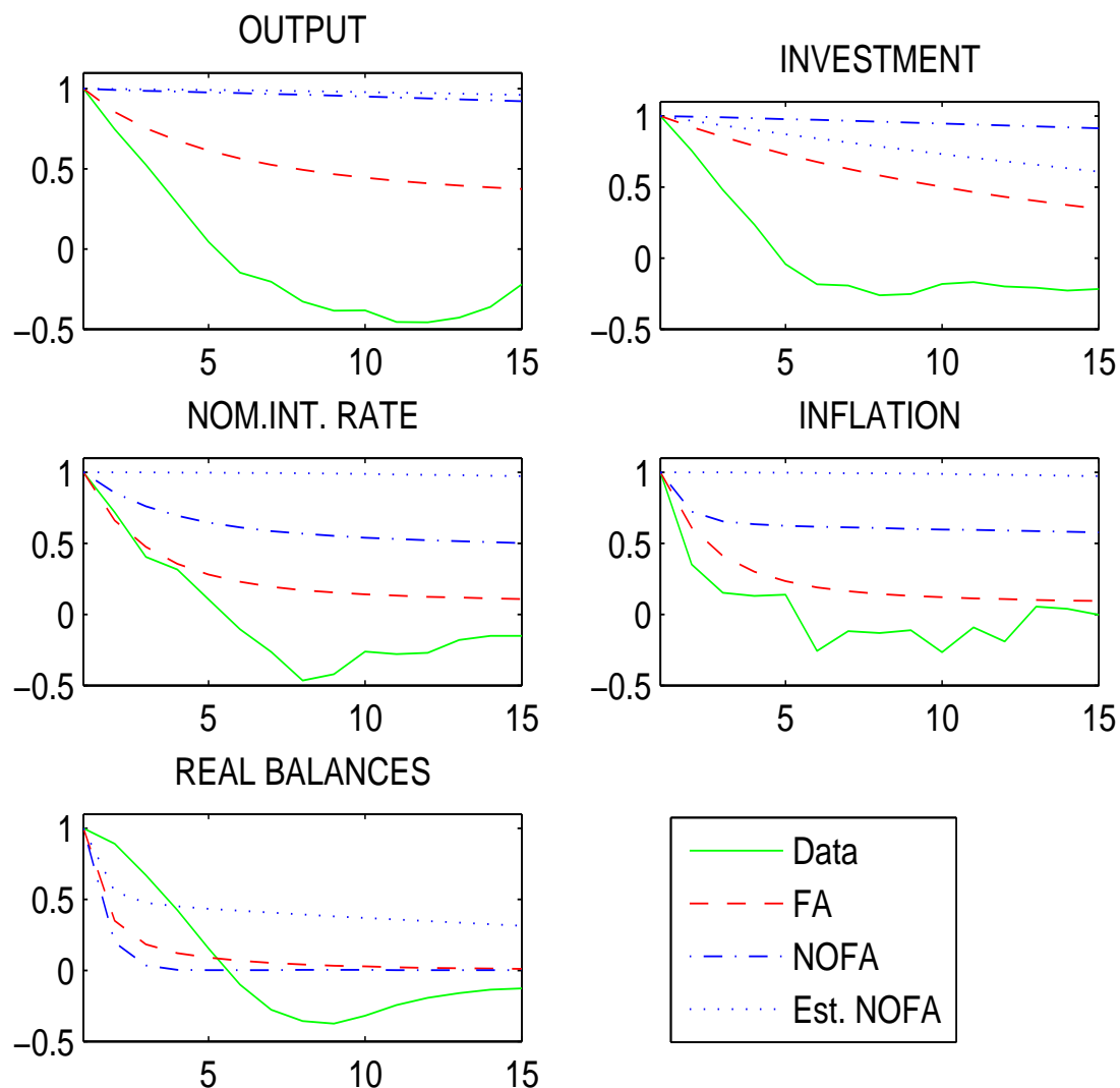
Figure 6: Autocorrelations
