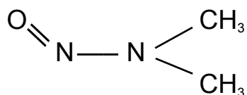
FIGURE 1 Chemical structure of NDMA
