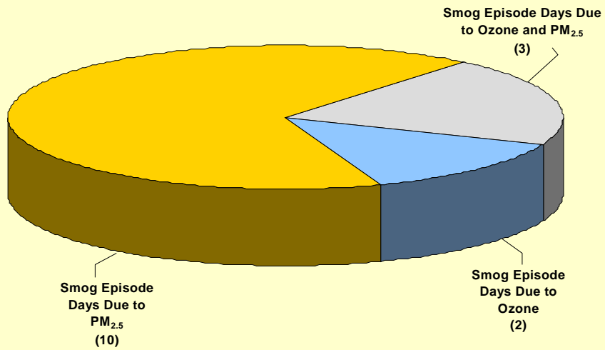
Figure 5.6a Smog Episode Days in Ontario (2004)
