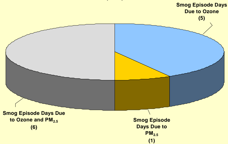
Figure 5.6b Smog Episode Days in Ontario (2003)
