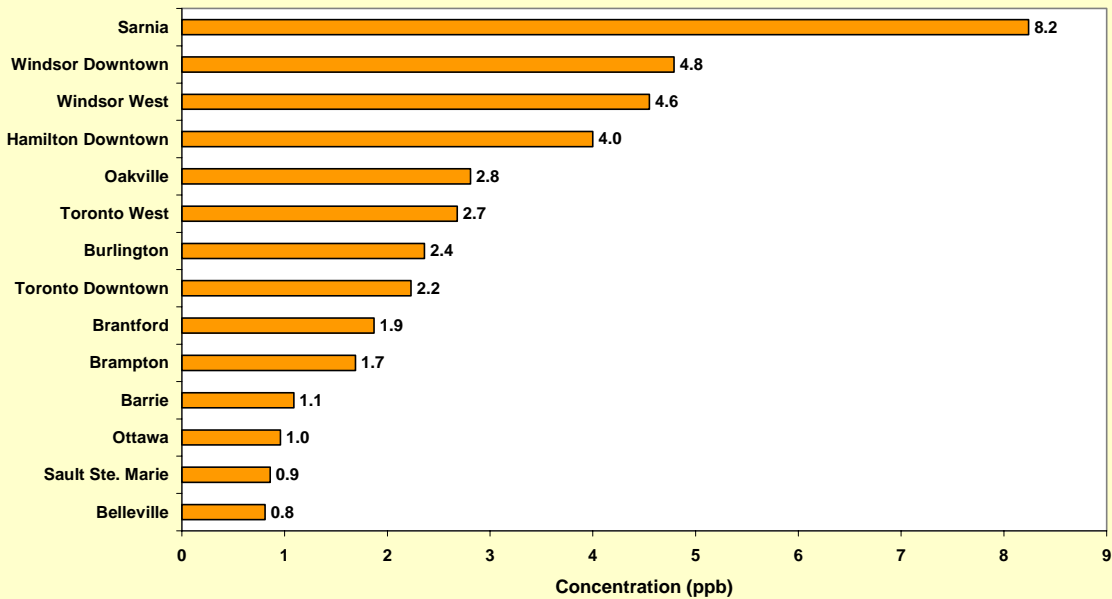
Figure 4.8 Sulphur Dioxide Annual Means Across Ontario (2004)
