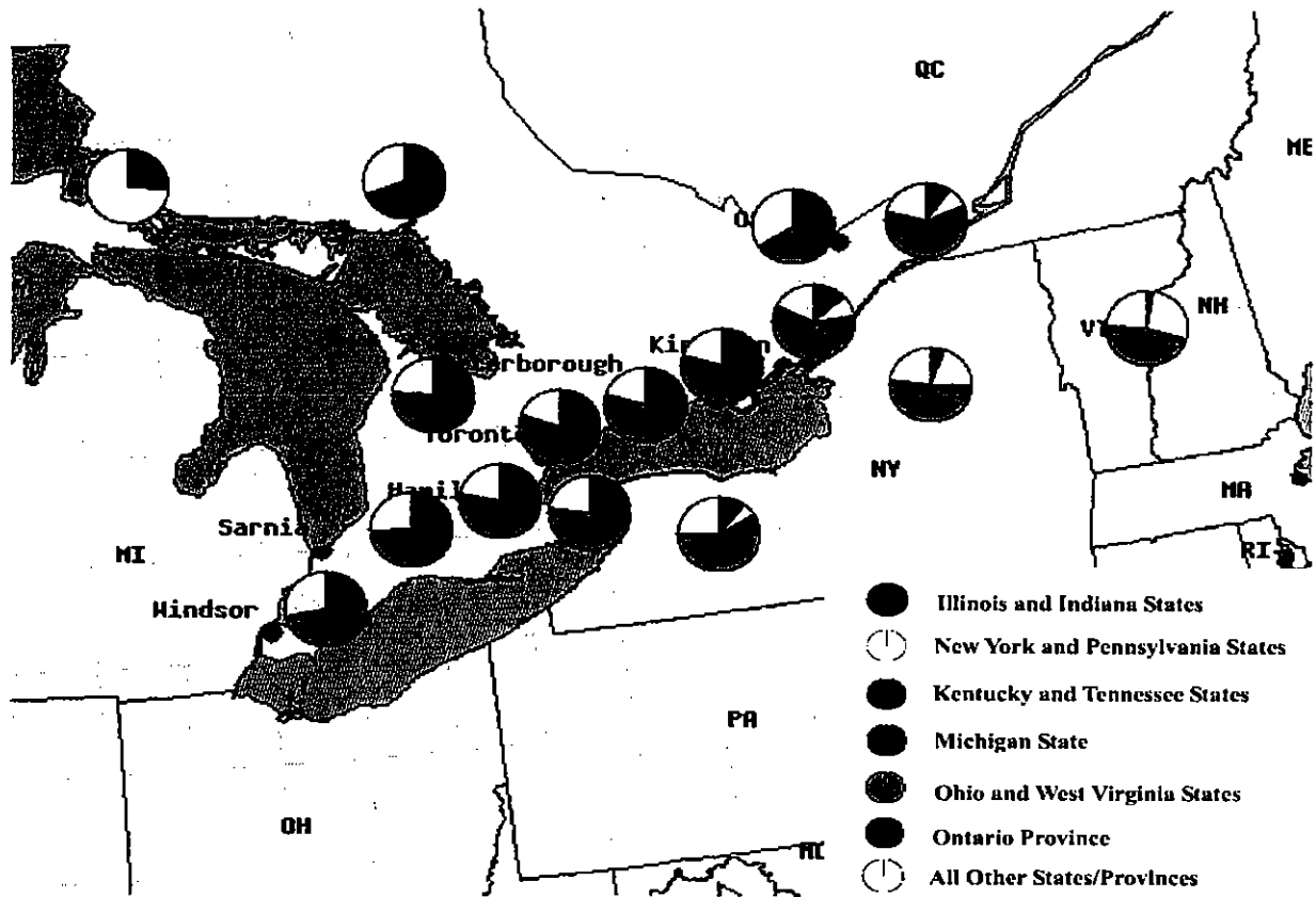
Figure 5: Regional Contribution to Sulphate at Selected Sites for Predicted Average on July 16, 1998 (Source: Ontario Ministry of Environment)
