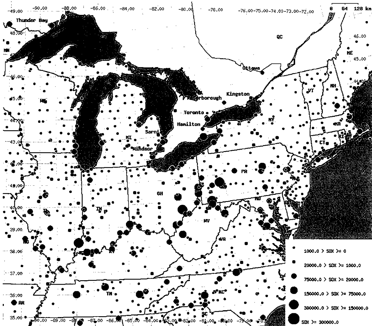
Figure 4: Comparative Sulphur Dioxide Emissions from Power Plants (Source: EPA 1995 Emission Inventories with 2001 Updates, Ontario 1999 Emission Inventories)
