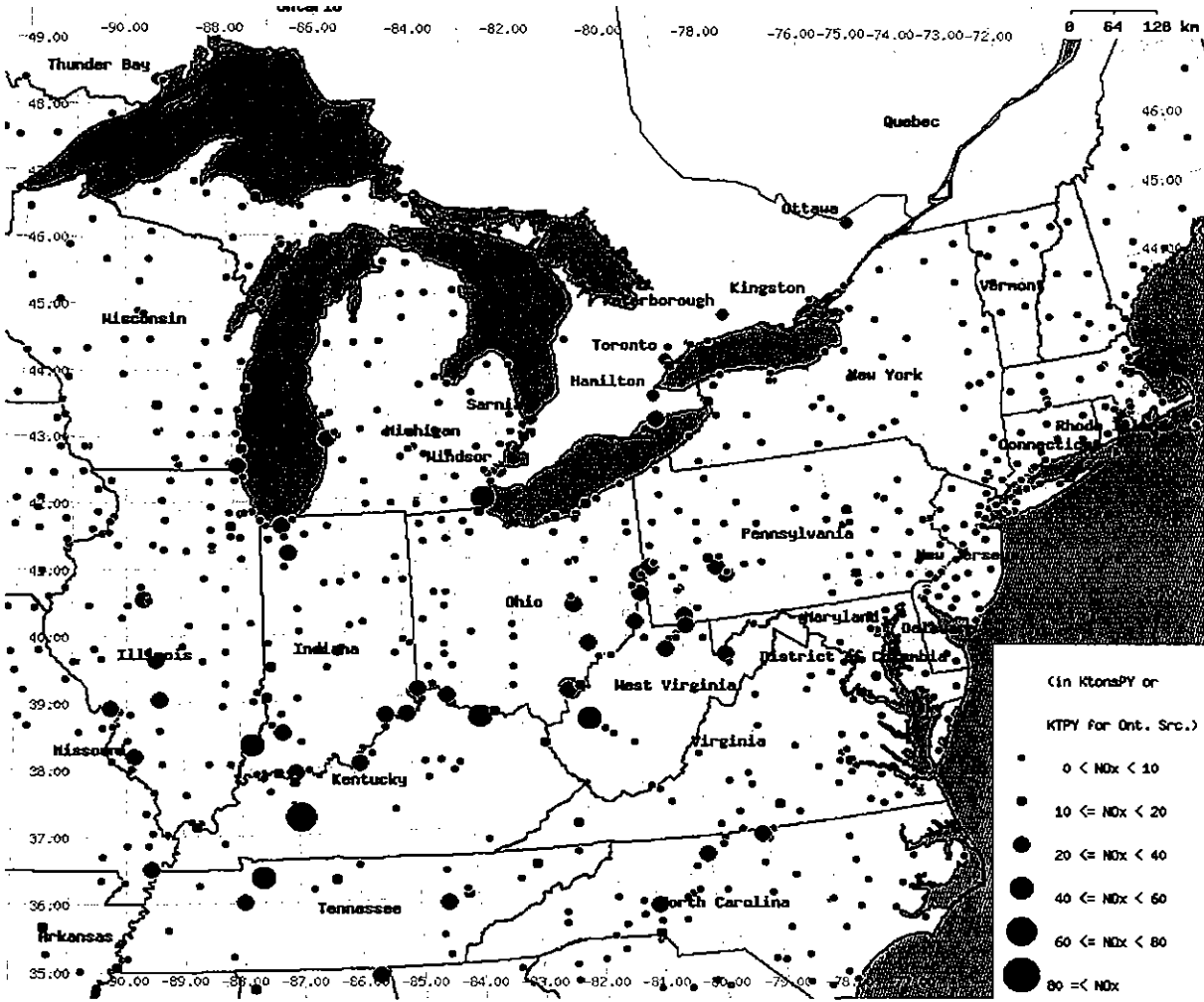
Figure 3: NOx Emissions from Power Plant Sources in Eastern U.S. and Southern Ontario (Source: EPA and Ontario Emission Inventories 1995, 1999 and 2001)
