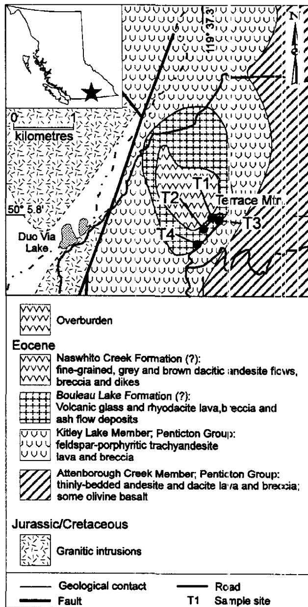
Figure 1. Location and geology of the Terrace Mountain hydrated obsidian deposit (modified from Church, 1980).
