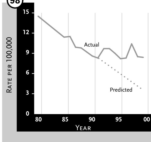
Figure 98 Tuberculosis Rates B.C., 1980-1999
