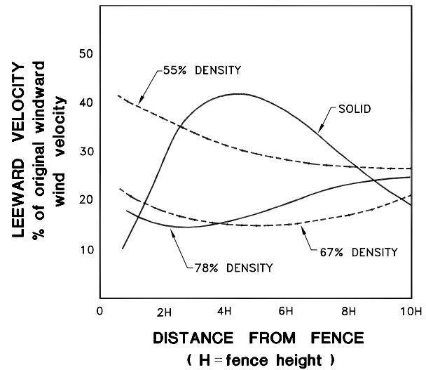
Figure 2 Wind velocity reduction from windbreak fences
