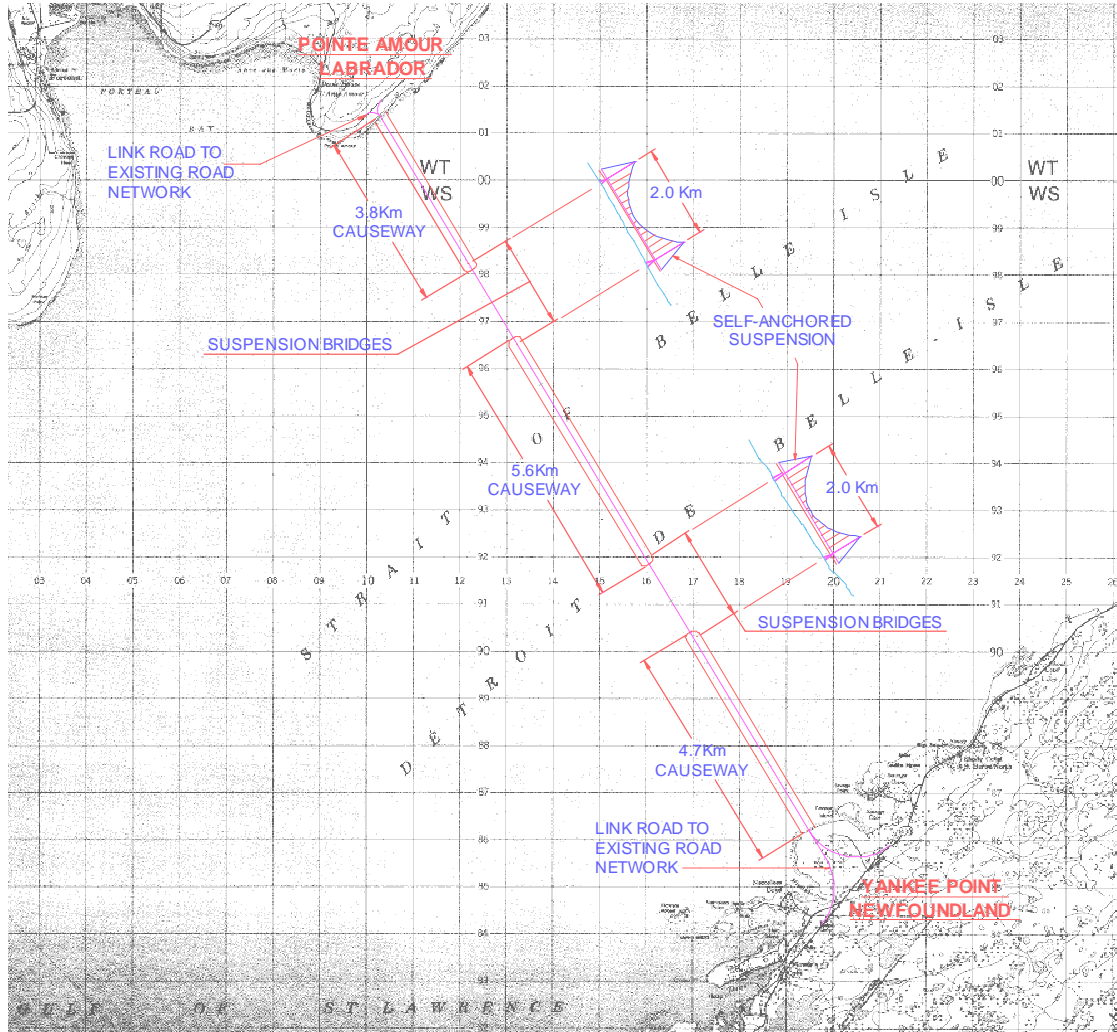
Figure 4.3 Causeway Arrangement
