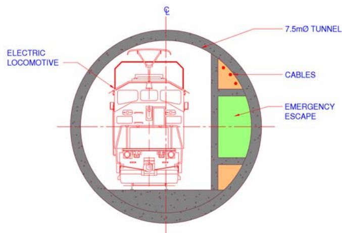
Figure 4.9 - TBM Bored Rail Tunnel - Conceptual Cross Section
