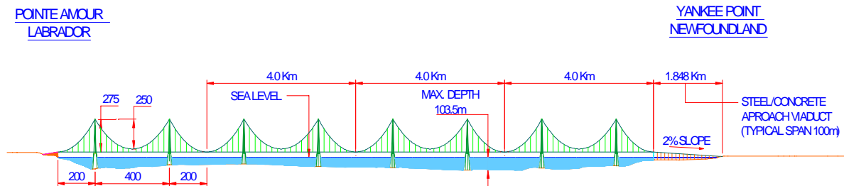
Figure 4.1 Suspension Bridge Concept
