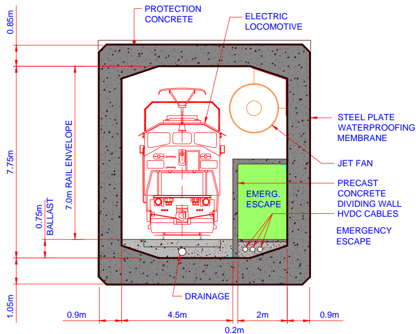
Figure 4.26 - ITT Rail Tunnel Cross-section
