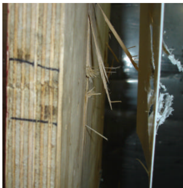
Figure 4.3: Typical failure of Original Warning Shot Target, Post Impact Side view
