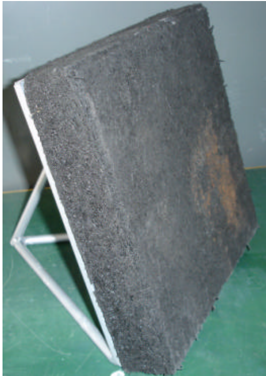
Figure 2.1: Alternative Target Type 1: Recycled Rubber with \frac{1}{4} " AR500 Steel backing
