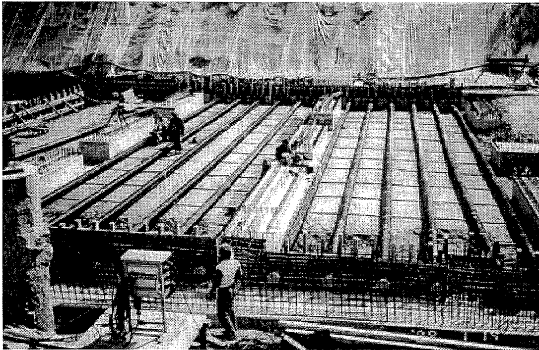
Figure 2-2: Piping layout during construction of a ground coupling system
