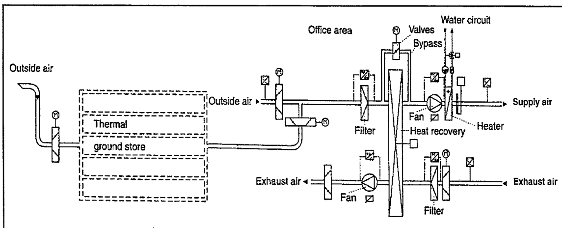
Figure 2-1: Schematic of an HVAC system with ground coupling
