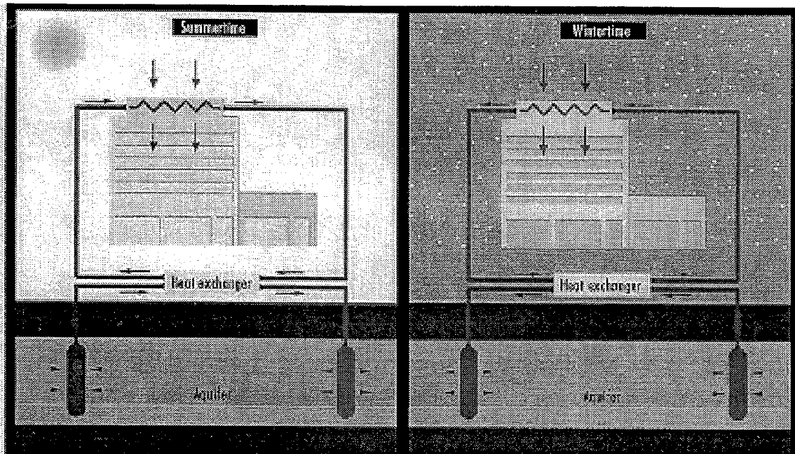
Figure 8-1: Schematic of a ground cooling with water system
