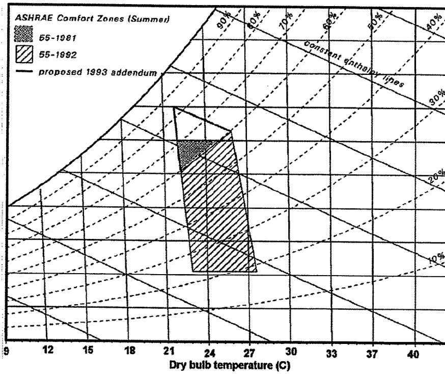
Figure B-1a: ASHRAE Standard 55 (ASHRAE psychrometric chart)
