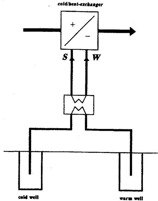
Figure 8-2: Direct ground water cooling
