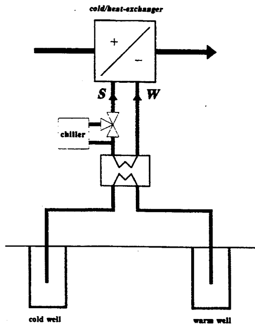
Figure 8-3: Direct ground water cooling with additional cooling
