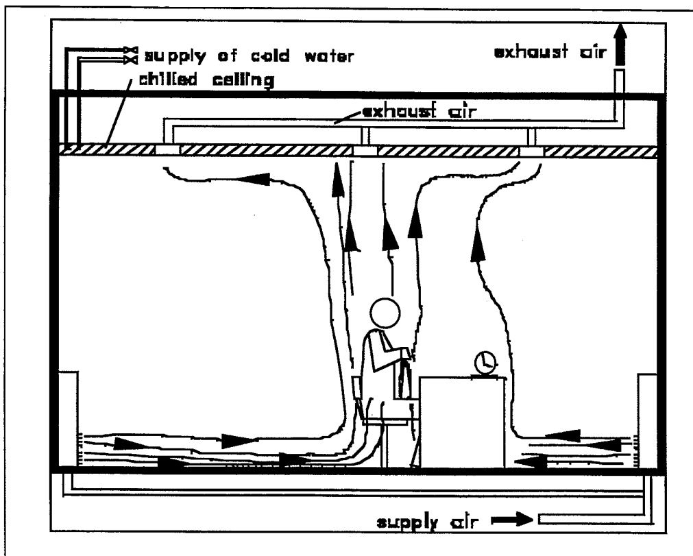
Figure 7-1: Cooling system using chilled ceilings and displacement ventilation
