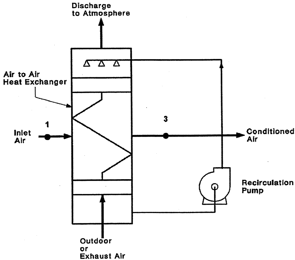
Figure 5-2: Indirect evaporative cooling system
