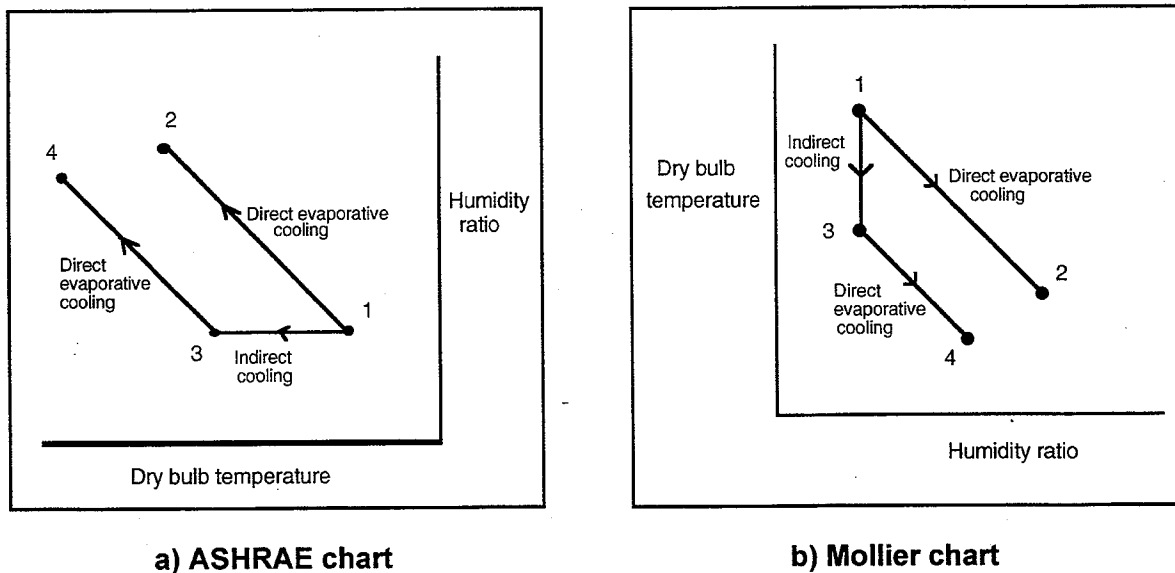
Figure 5-4: Evaporative cooling processes on the psychrometric chart
