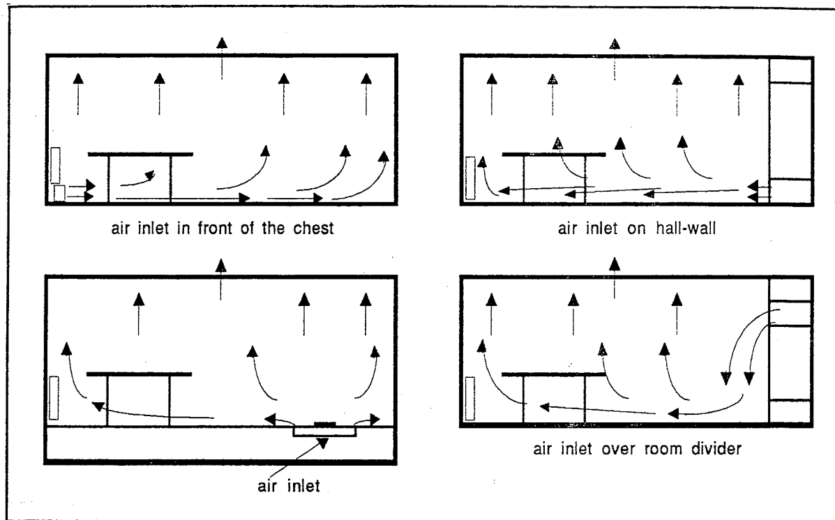
Figure 7-2: Various configurations for air inlet for displacement ventilation
