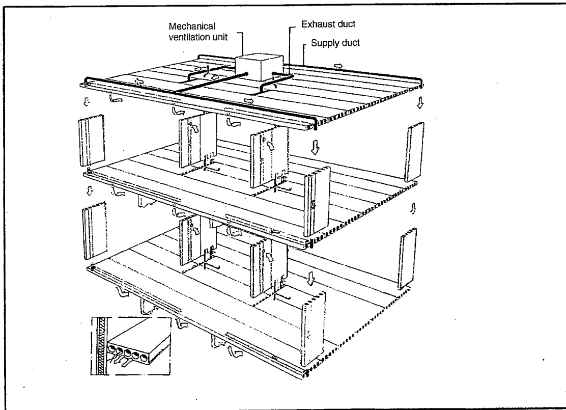
Figure 3-1: Air exchange ductwork integrated with the building construction (reference: EBES, VTT publications, Number 537, Espoo, Finland, 1988)
