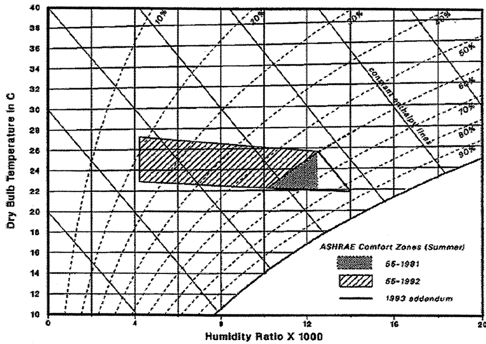
Figure B-1b: ASHRAE Standard 55 (Mollier chart)
