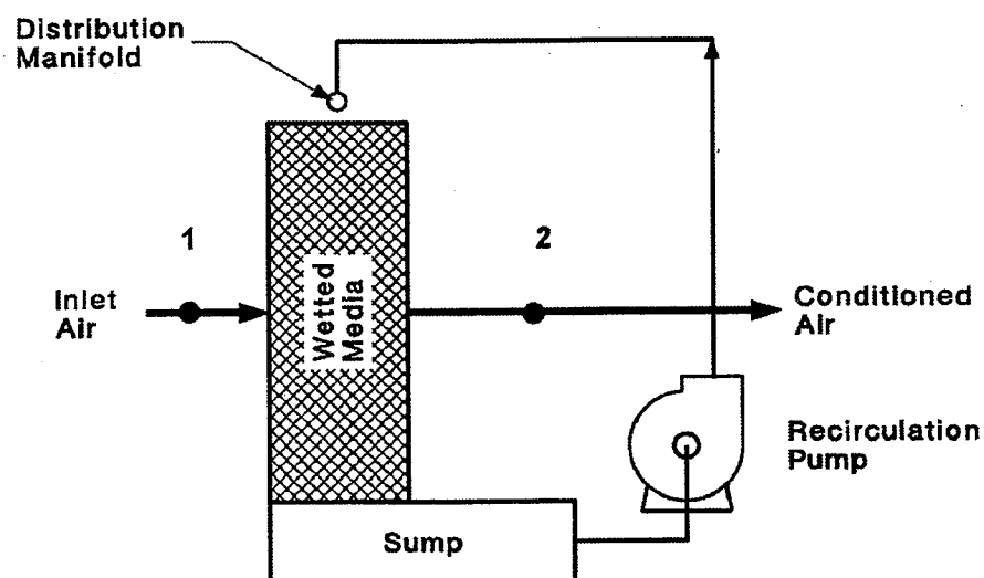
Figure 5-1: Direct evaporative cooling system
