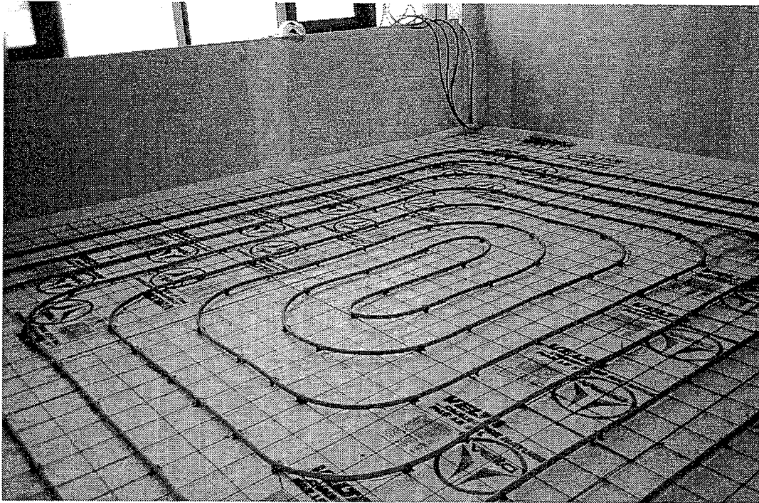
Figure 6-2: Slab cooling piping network before being embedded in concrete
