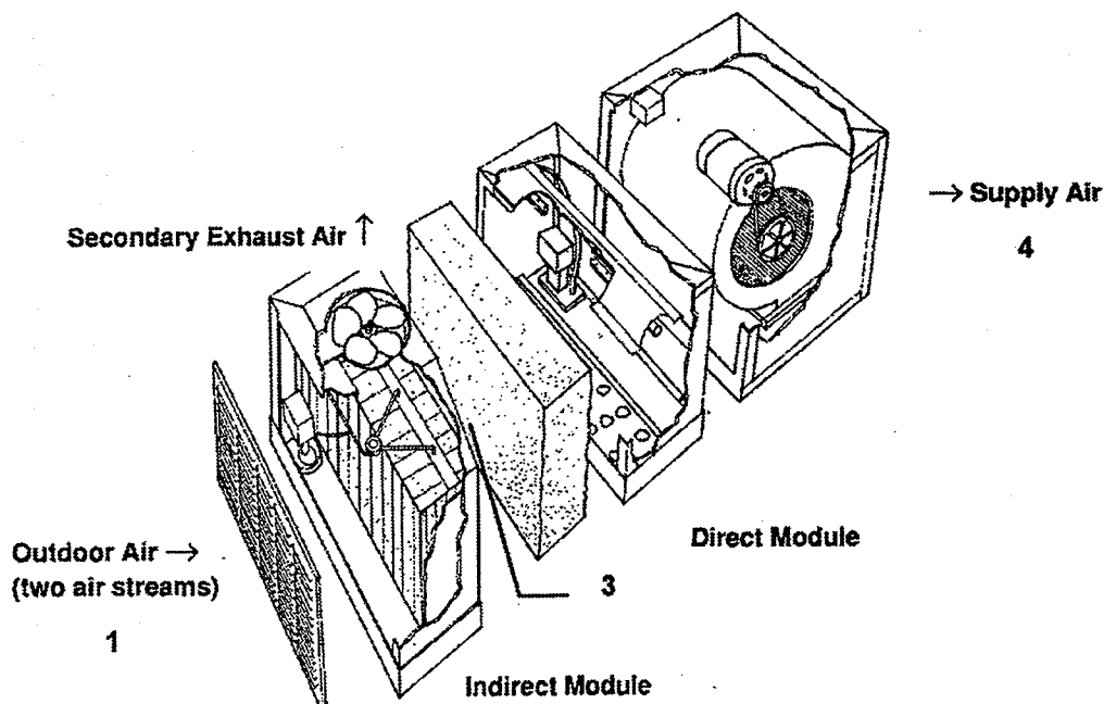
Figure 5-3: Two stage indirect/direct evaporative cooling system
