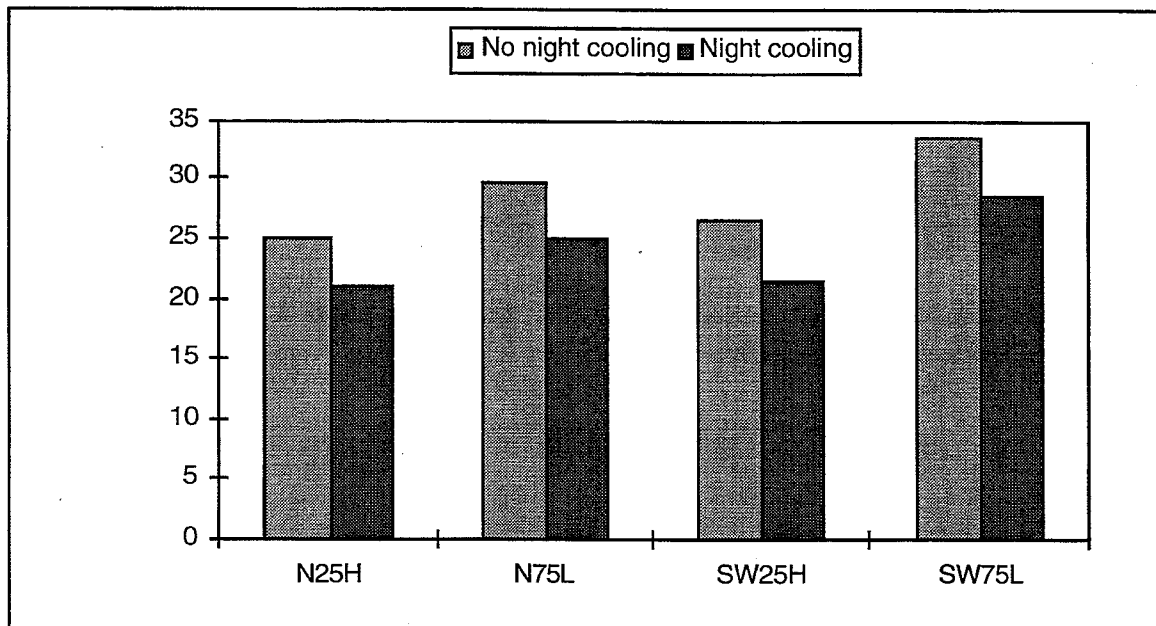
Figure 1-1: Peak temperatures in buildings with and without night cooling
