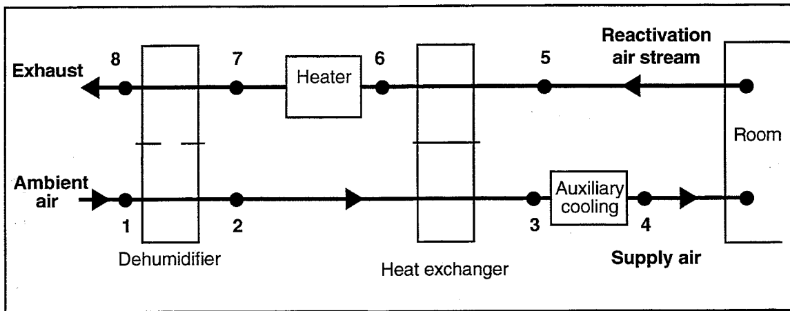
Figure 4-1: Schematic of a solid desiccant cooling system
