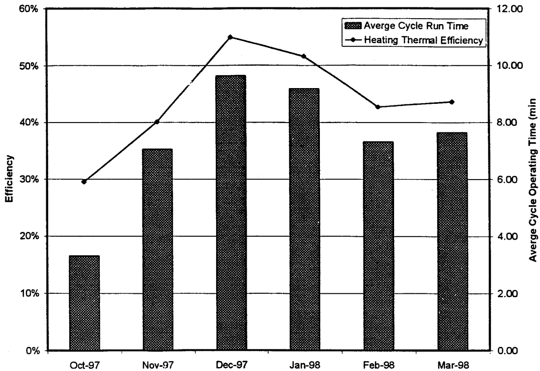
Figure 5.2: Boiler Thermal Efficiency vs. Average Cycle Run Time
