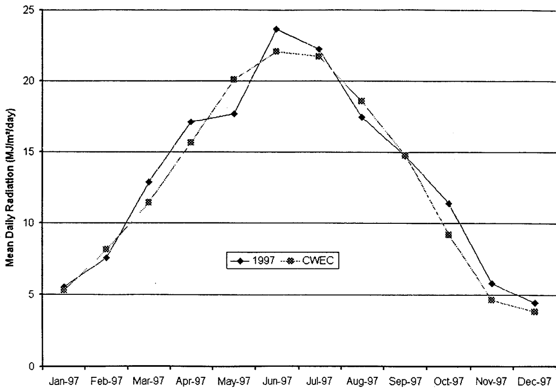
Figure 4.2: 1997 and CWEC Global Horizontal Solar Radiation
