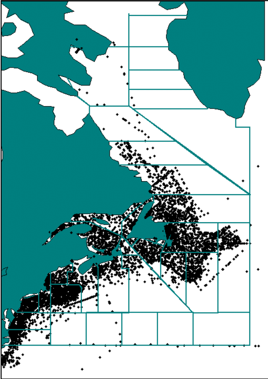
Figure 5. Delayed mode profile stations 2004. Total = 7764 Stations
