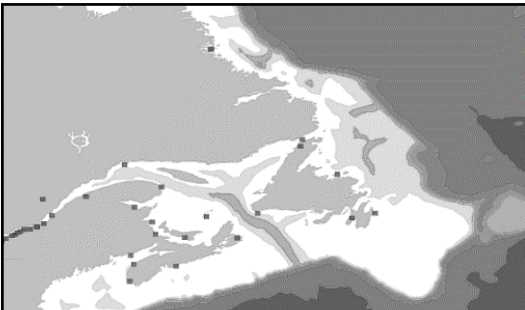
Figure 9 Tide and water level data in the NAFO Area in 2004
