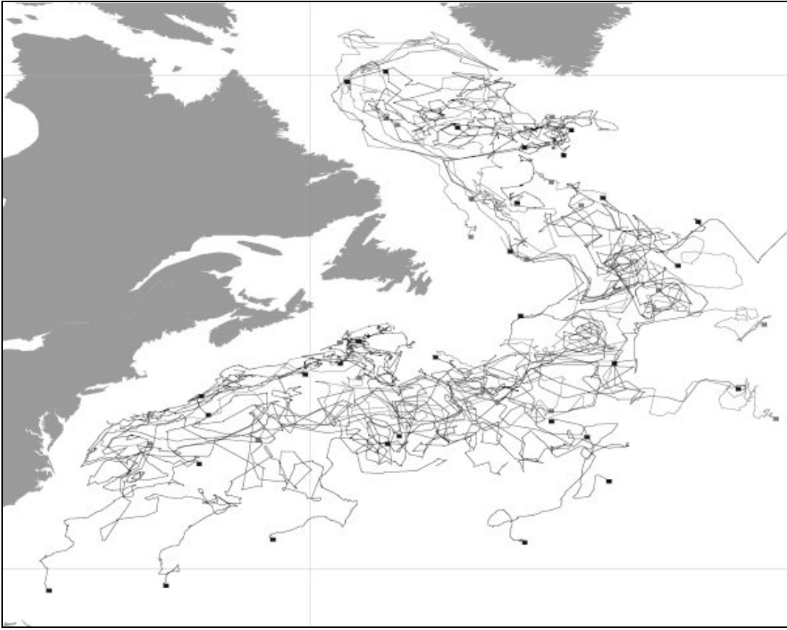
Figure 1: Canadian Argo profiling floats May 2005
