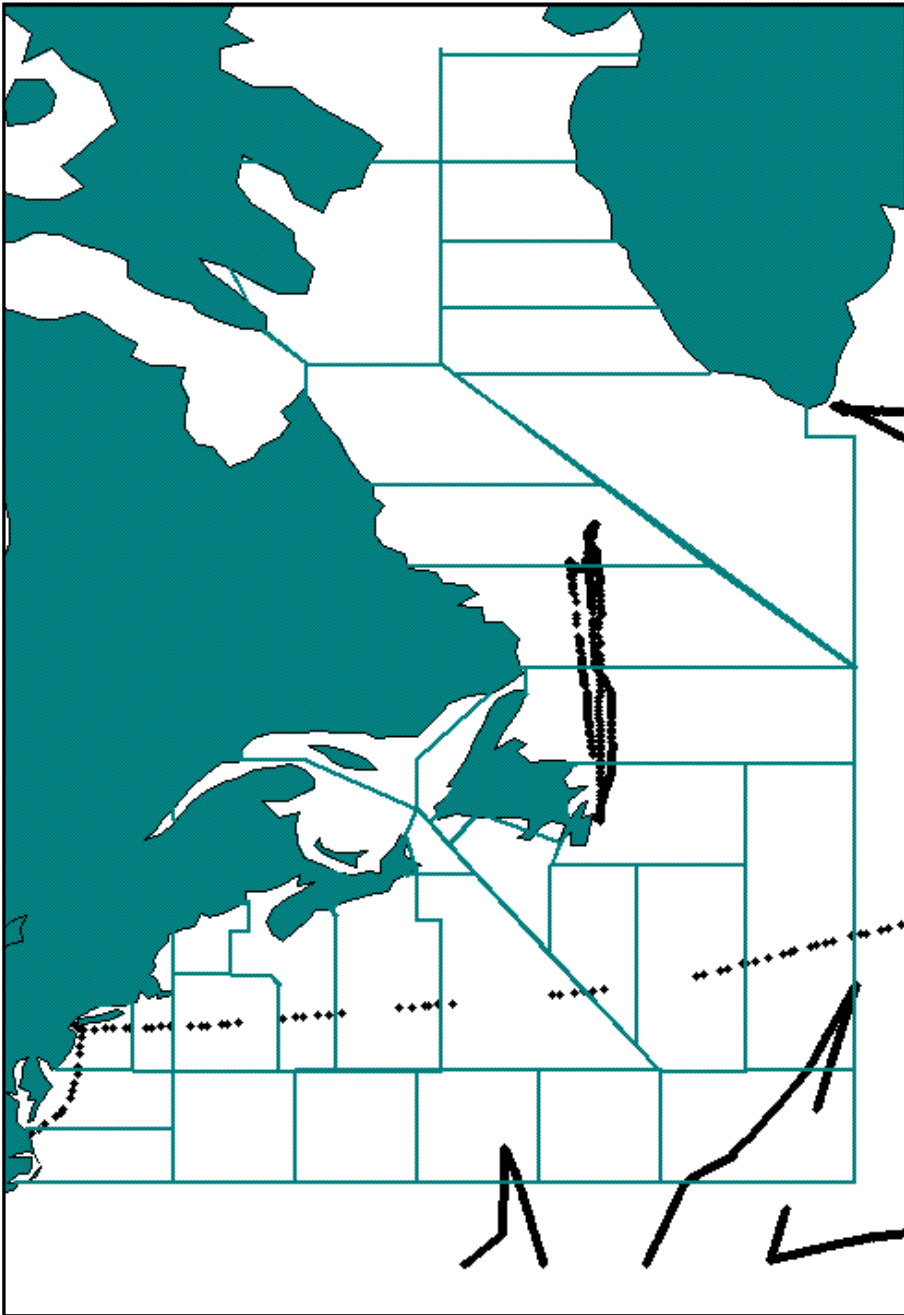
Figure 4. Surface Thermosalinograph stations 2004 Total = 1191 Stations
