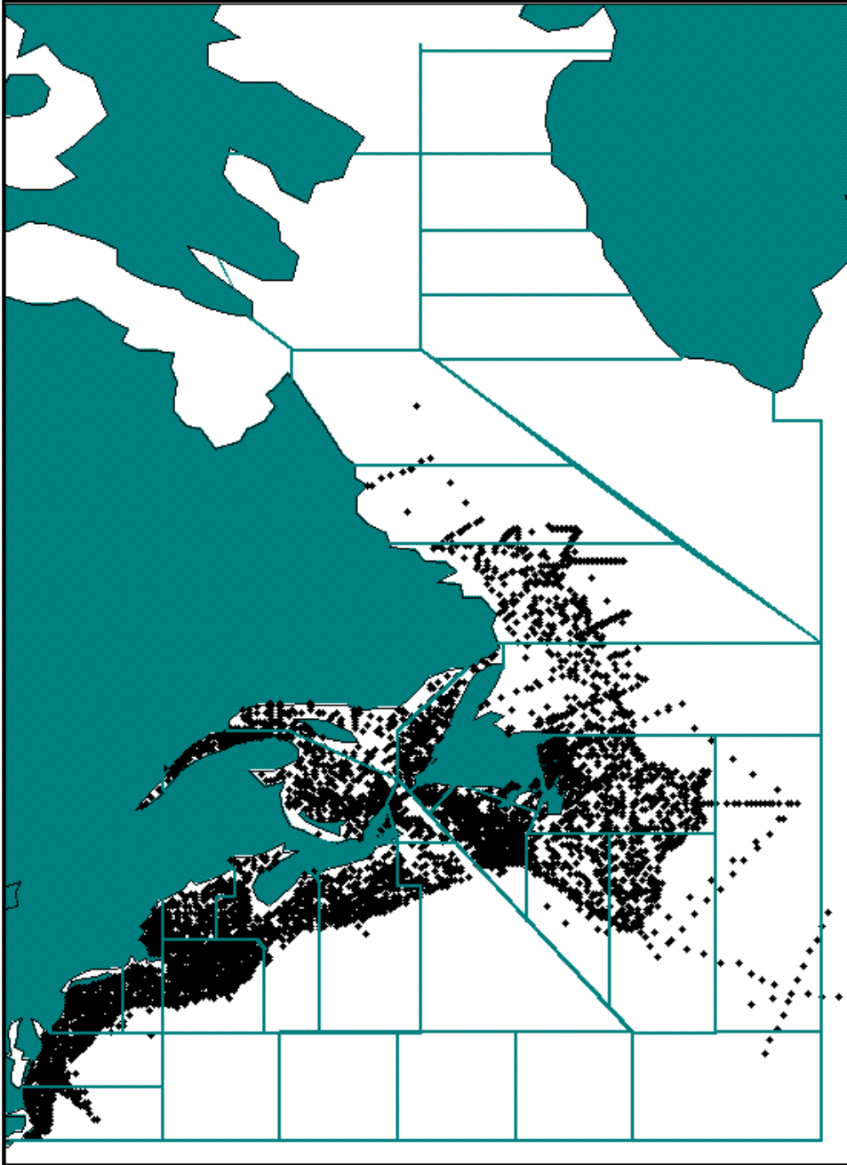
Figure 6. Delayed mode profile stations collected before 2004 and processed in 2004. Total = 9399 Stations
