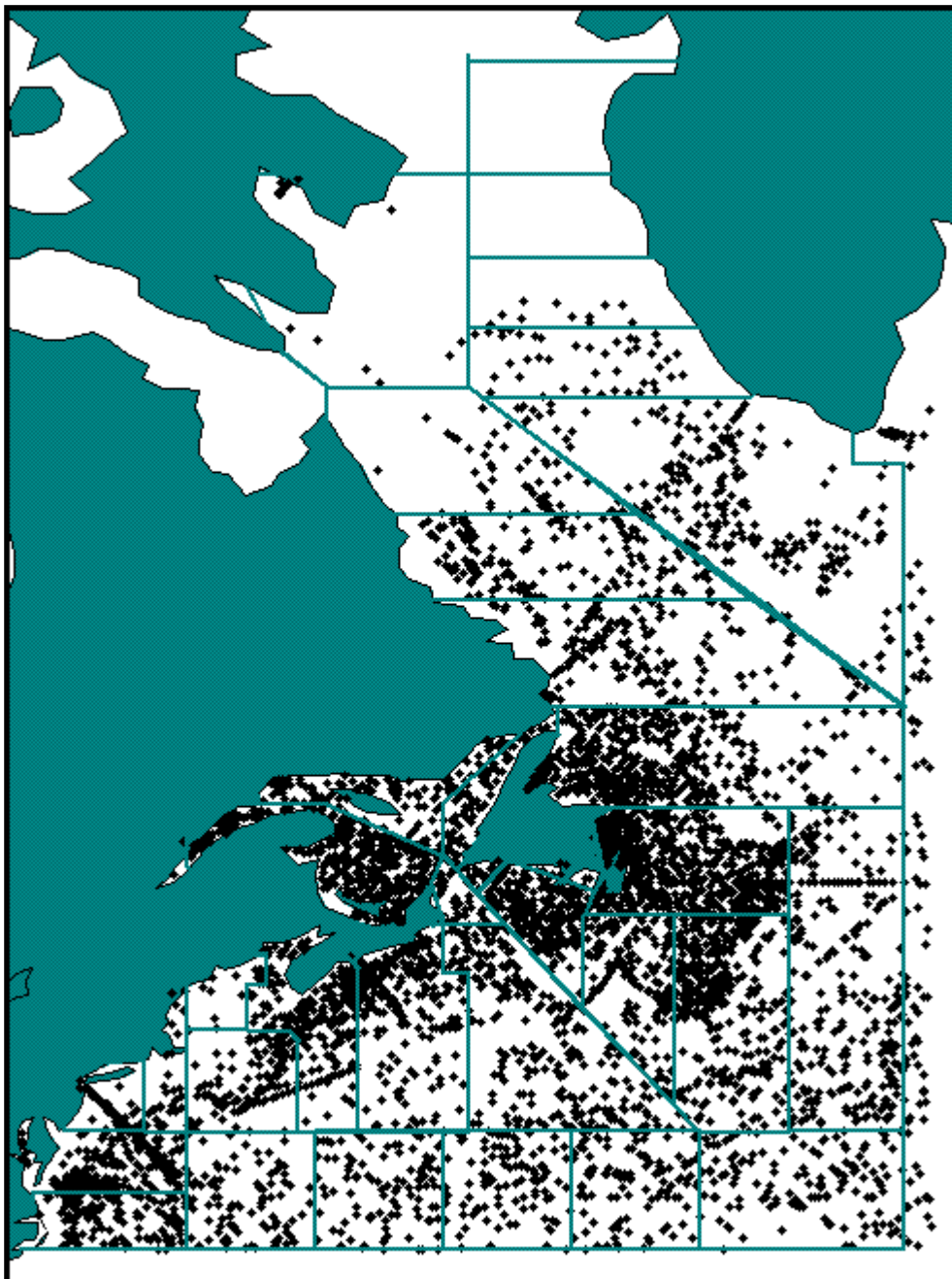
Figure 3. Real Time Temperature-Salinity Stations 2004 Total = 65666 Stations
