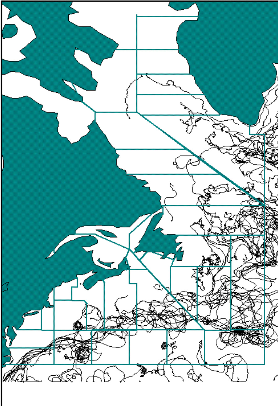
Figure 7. Drifting Buoy messages 2004. Total = 84106 Messages
