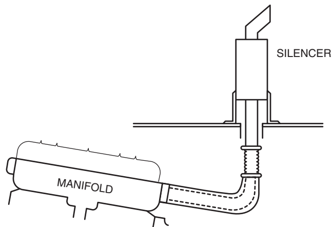
Figure A4-1 Typical Dry Exhaust System
