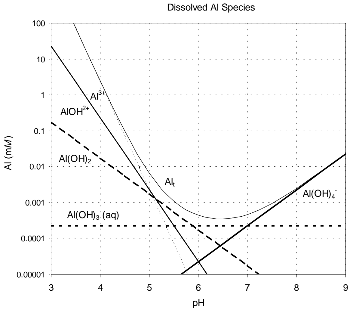
Figure 1. Solubility of aluminum species (and total aluminum, Al_t ) in relation to pH in a system in equilibrium with microcrystalline gibbsite (0.001 mM = 0.027 mg/L).
